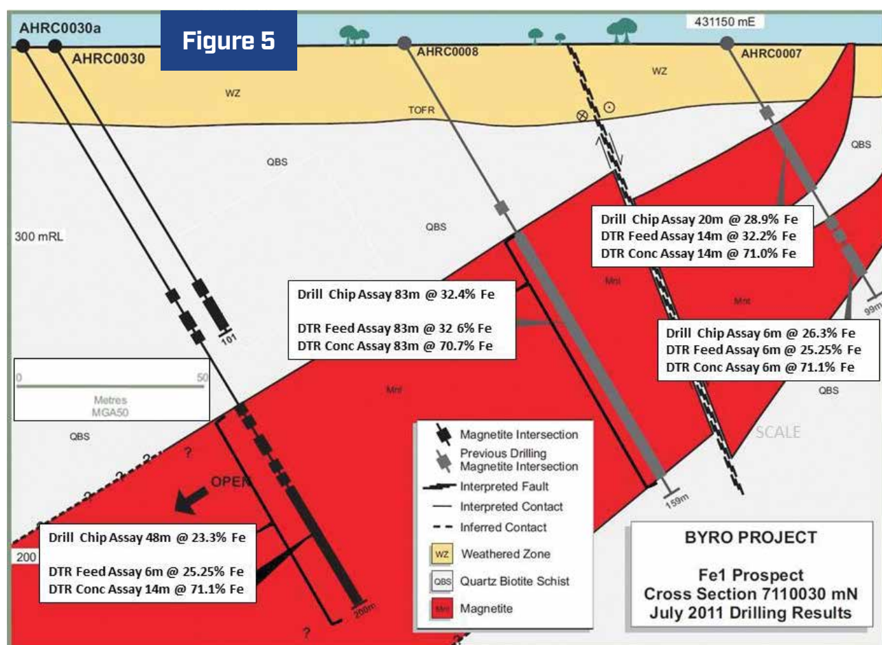
Fe1 Crosssection
