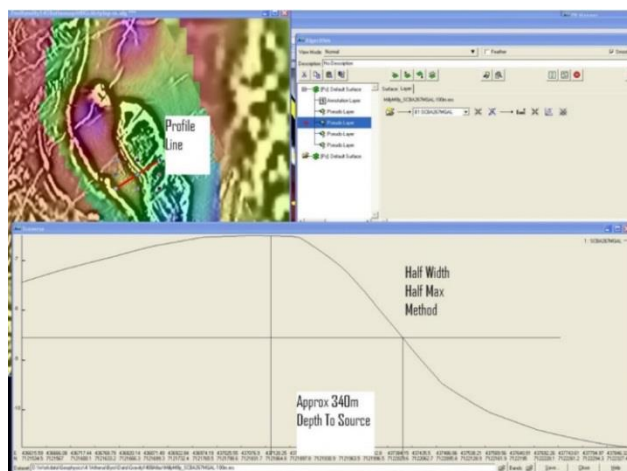
Figure 6. Gravity anomaly depth interpretation at AHDH0007
