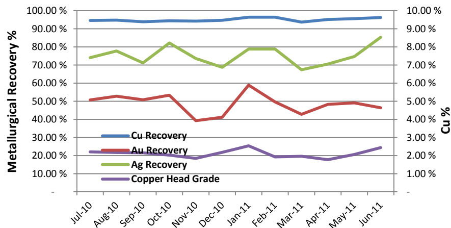
Tritton Plant Recoveries - 2011FY.
