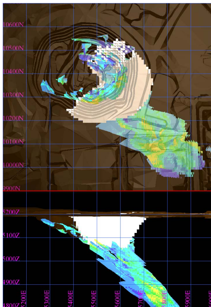
Figure 2 Murrawombie open pit extension plan and section, (extension mining shown in light pink)
