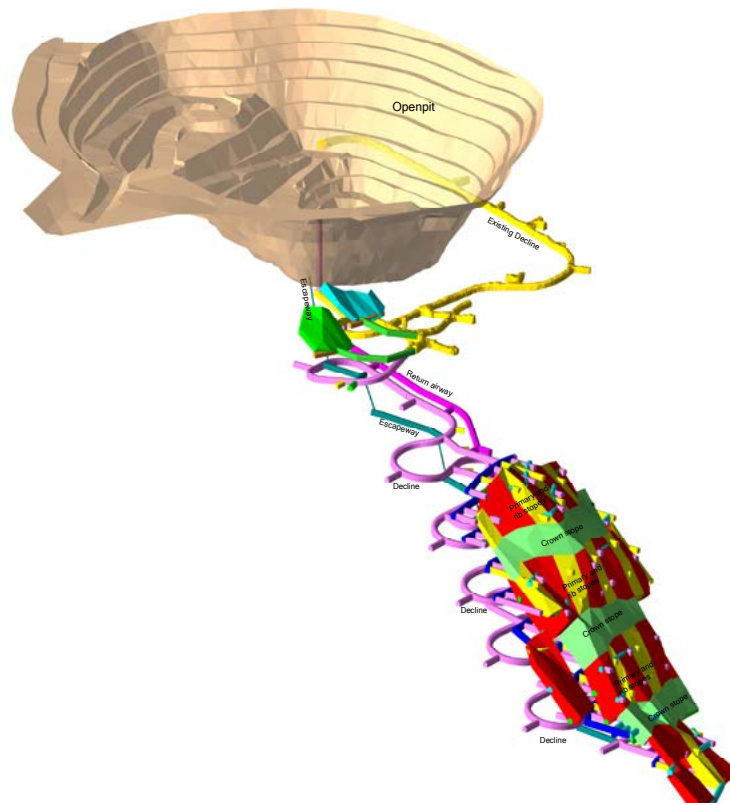
Historical Murrawombie open pit with current and planned underground mining
