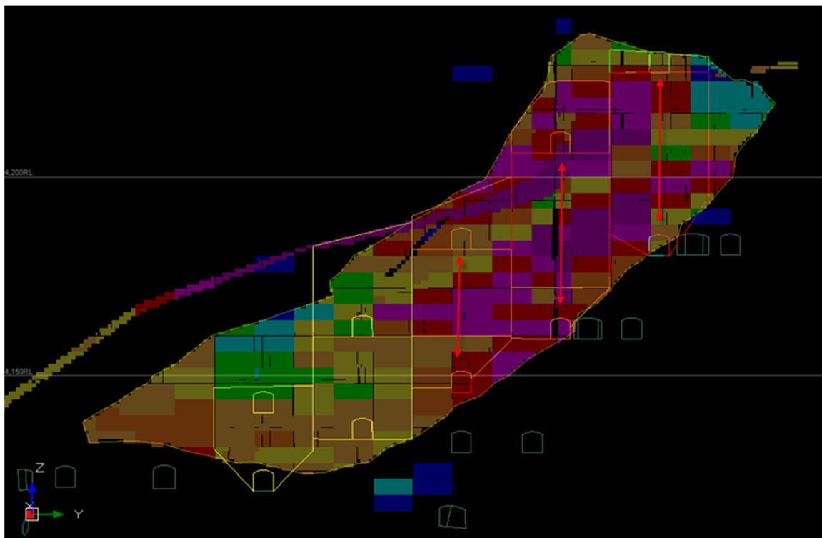
Figure 8 Typical section showing tall and vertical stopes with trough undercut design
