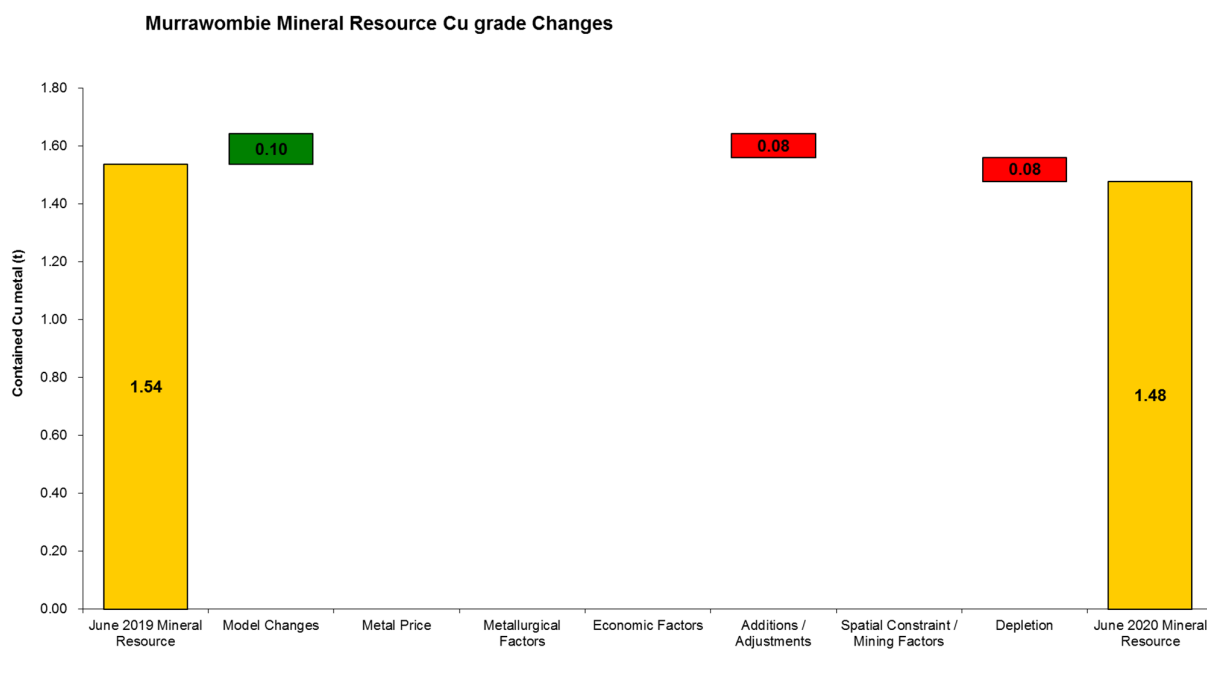
Figure 5: Copper grade changes between the 30 June 2019 mining position and 30 June 2020 mining position at the Murrawombie deposit. Figures are reported from raw data and rounded to nearest 0.01% Cu.
