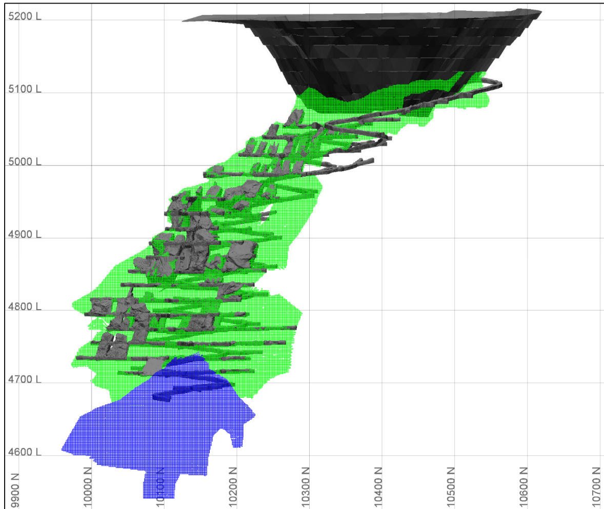
Figure 2: Long section view looking west at the reported Murrawombie deposit Mineral Resource at 30 June 2020 position (green solid – Indicated, blue solid – Inferred and grey solids – 30 June 2020 depletion wireframes).
