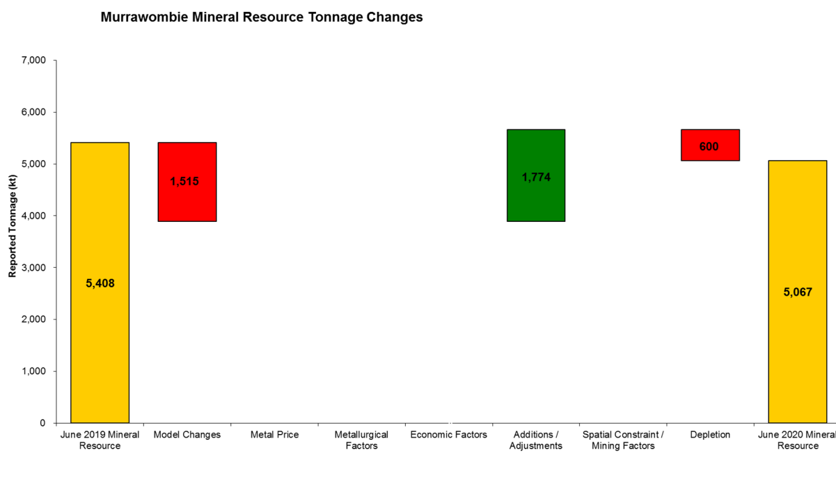
Figure 4: Tonnage changes between the 30 June 2019 mining position and 30 June 2020 mining position at the Murrawombie deposit. Figures are reported from raw data and rounded to nearest 1kt.
