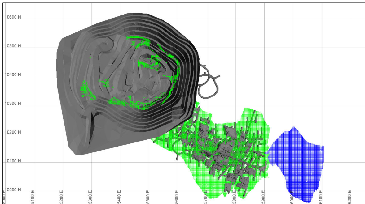
Figure 3: Plan view showing the reported Murrawombie deposit Mineral Resource at 30 June 2020 position (green solid – Indicated, blue solid – Inferred and grey solids – 30 June 2020 depletion wireframes).
