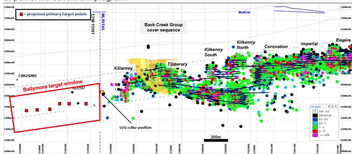
Figure 9 – Long section view showing location of proposed target points along the Ballymore fault as part of the current drill program.
