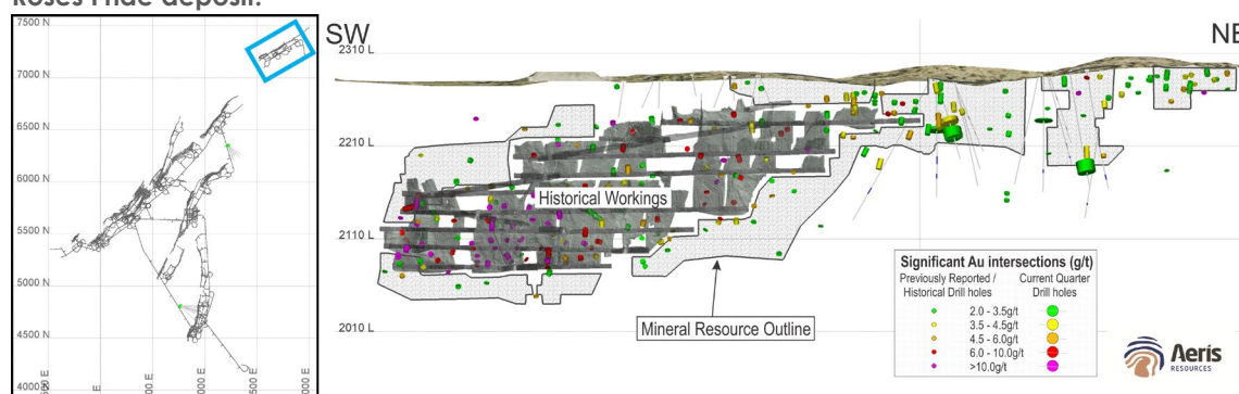
Figure 10 – Long section view showing location of RC drill holes completed during the quarter at the Roses Pride deposit.
