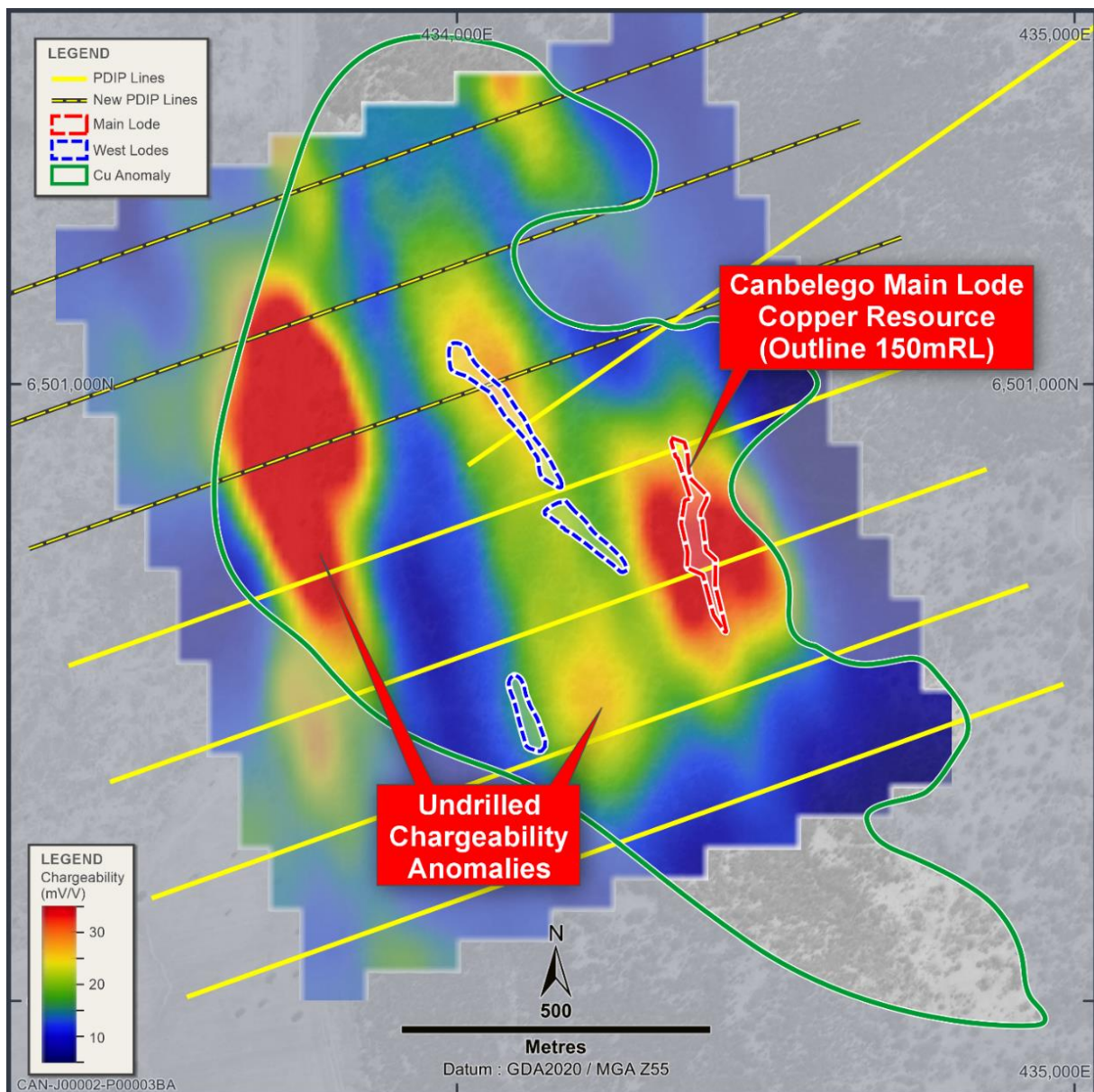
Figure 1 – Canbelego 3D inversion IP chargeability depth slice at 130mRL (175m below surface) and outline of anomalous surface copper geochemistry.
