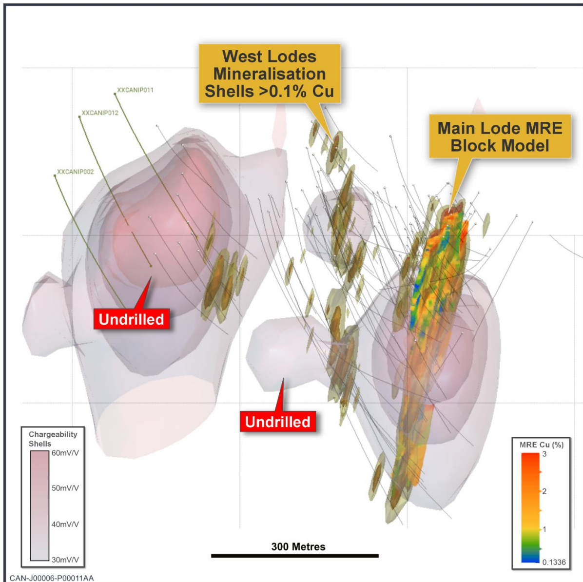
Figure 2 – Canbelego 3D inversion IP chargeability shells looking down towards the northwest, showing drilling, the Main Lode MRE block model 5 , the West Lodes >0.1% Cu mineralisation shells. Initially three drillholes are proposed to test the new undrilled Western IP anomaly (XXCAN labels).
