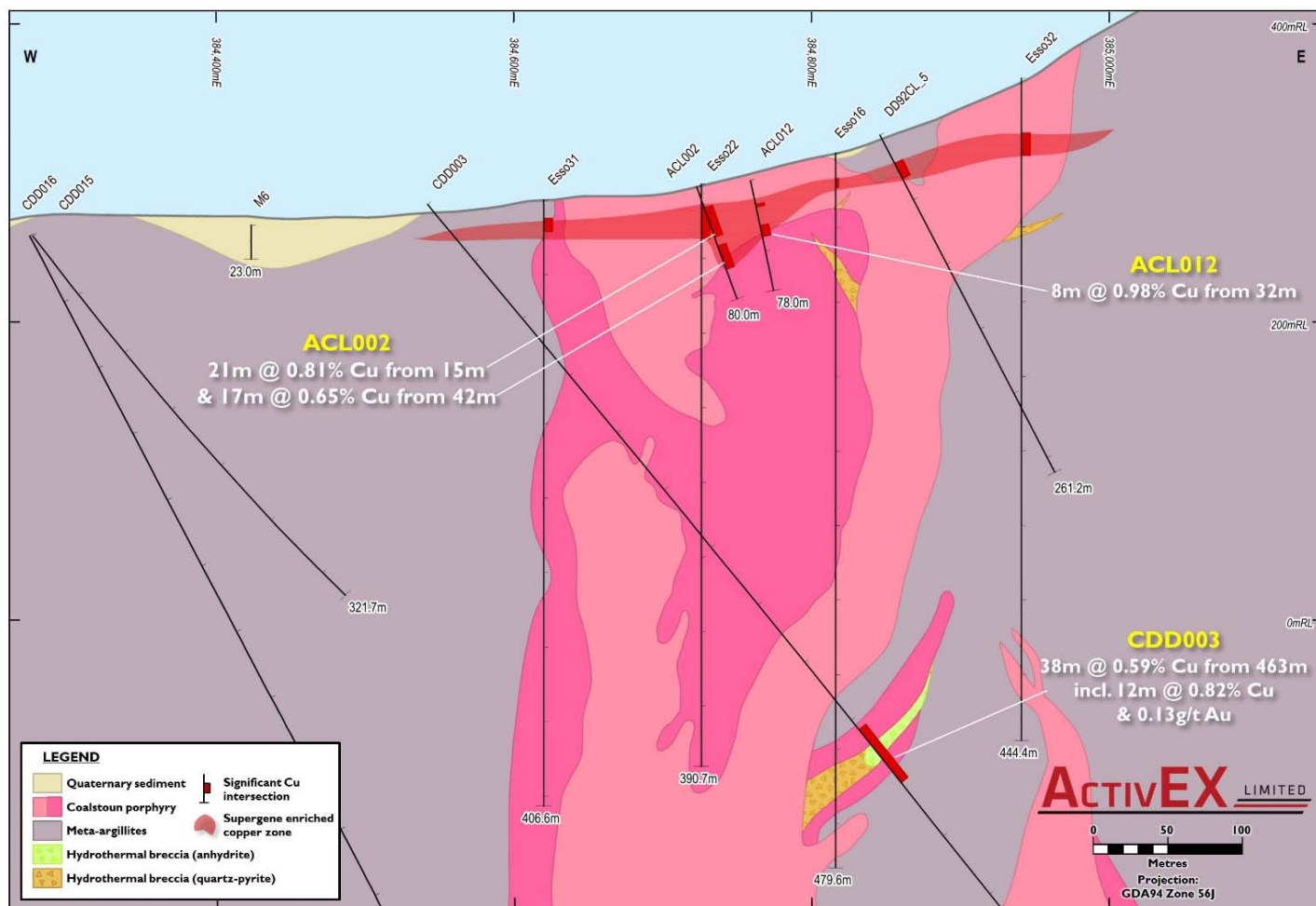
Figure 4. Drill cross section of ACL002, ACL012 and CDD003
