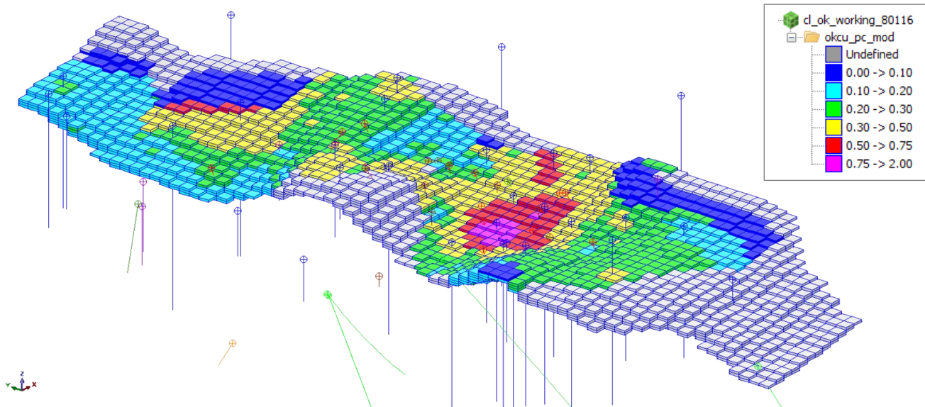
Figure 5: Copper block grade distribution for the supergene mineralisation
