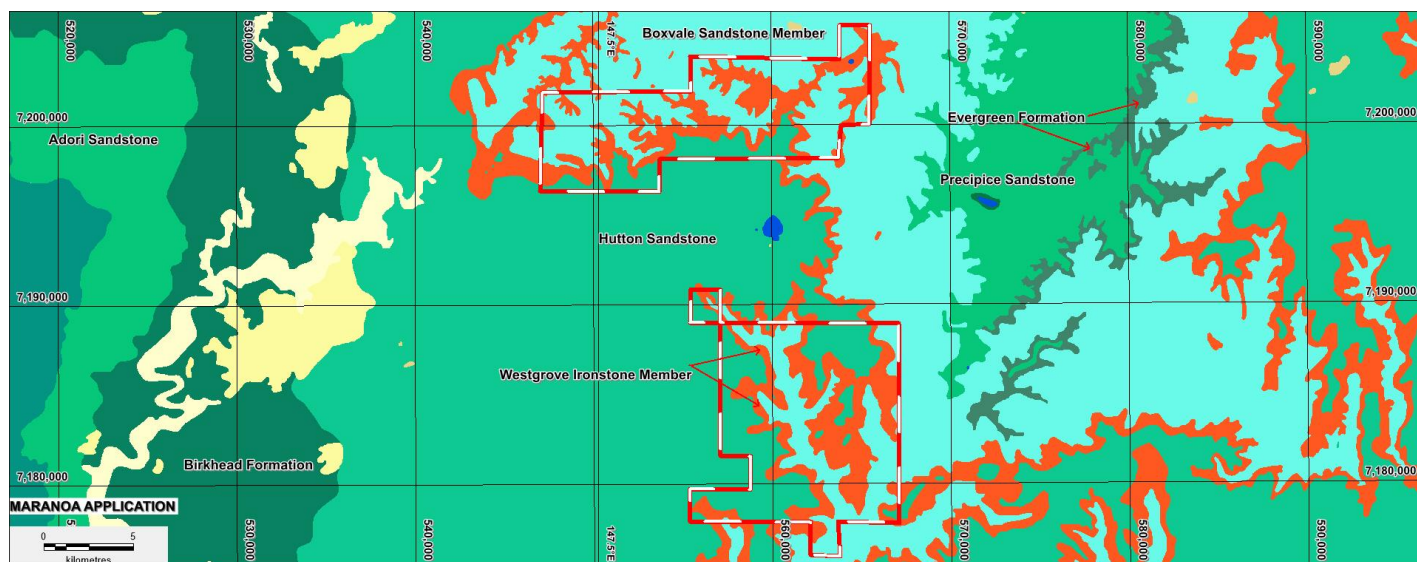
Figure 16. ActivEX Maranoa Local Geological Setting – Note the tenement application is targeting the Westgrove Ironstone Member
