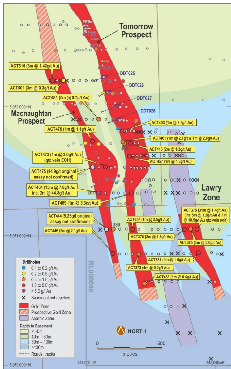
Figure 7: Macnaughtan, Tomorrow and Lawry Zones at Tandarra, with AC drill plan showing significant result (source: Catalyst Metals Ltd)
