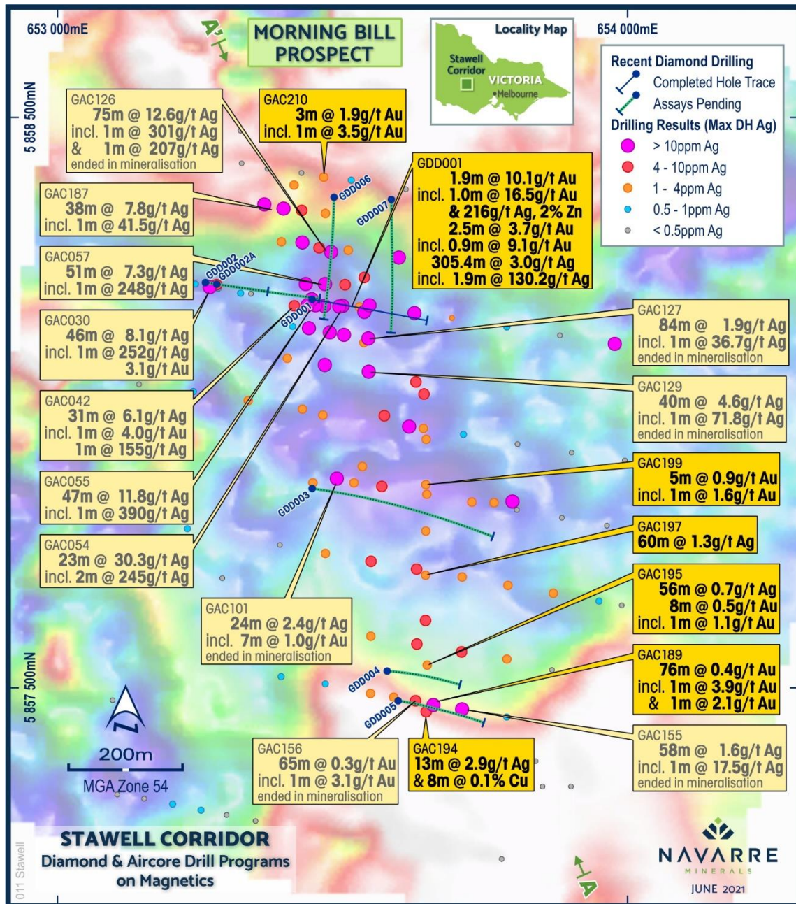
Figure 2: Plan of Morning Bill showing diamond and air core results and magnetic survey.
