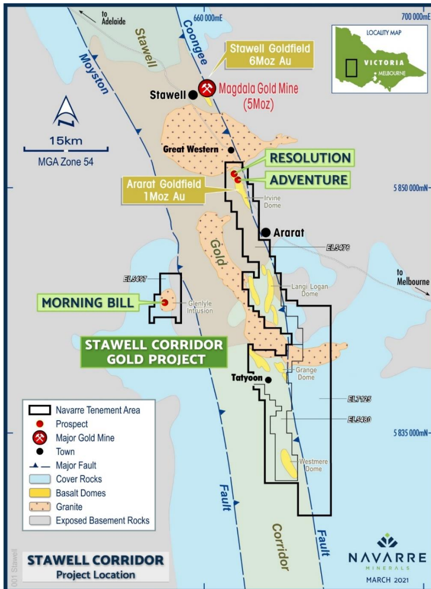
Figure 1: Location of Navarre's western Victorian gold projects.
