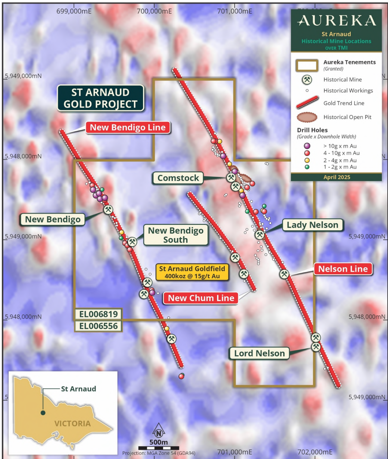
Figure 11 - Close-up of Shape-indexed TMI data overlain on historic Production centres within EL006819. Note correspondence between higher magnetic response and historical Mines. 14
