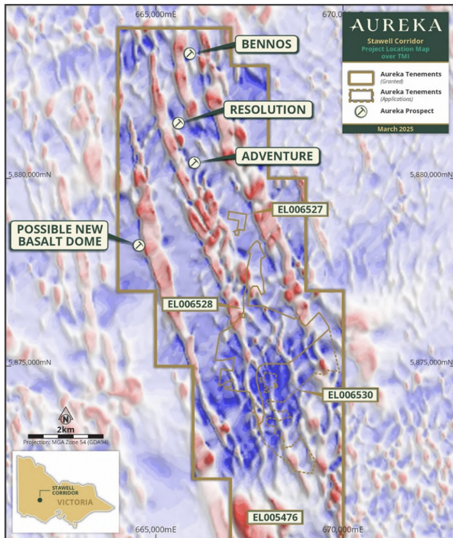
Figure 4 - Nordic geoscience's Shape indexed TMI Modelling showing Irvine, Benno and possibly new basalt domes on the western side. Resolution and Adventure gold lodes (which comprise the current JORC Resource) also marked.
