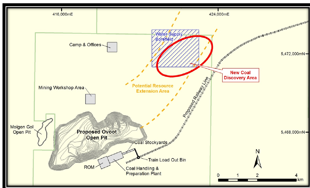
Figure 2: Proposed Ovoot Project Mine-Site Plan
