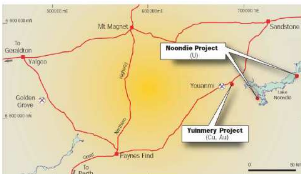
Figure 11. Location of Yuinmery project Figure from Empire Resources 2007 Annual Report
