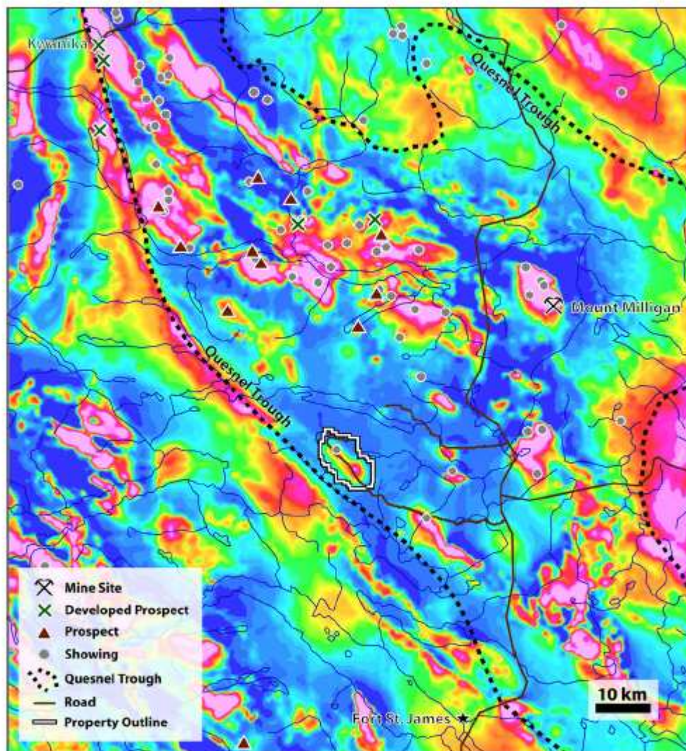
Figure 12. Location of the Inza property on regional magnetic image Figure from Strongbow website
