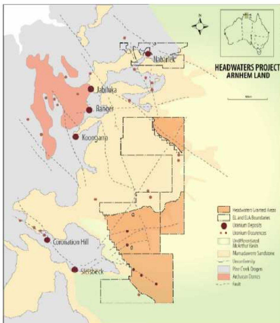
Figure 14. Location of the Headwaters project Figure from UEQ Report for the Quarter ended 31 March 2010
