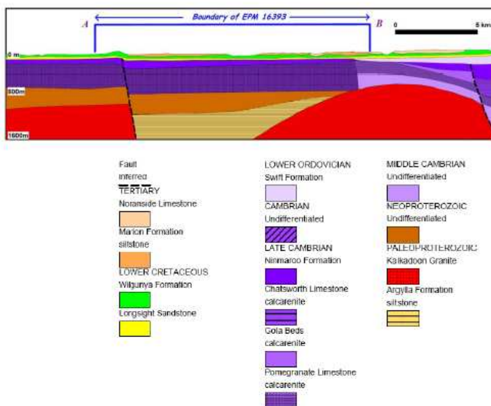
Figure 8. East-west section A-B through EPM 16393 Compiled by D G Jones from Casey et al (1967)
