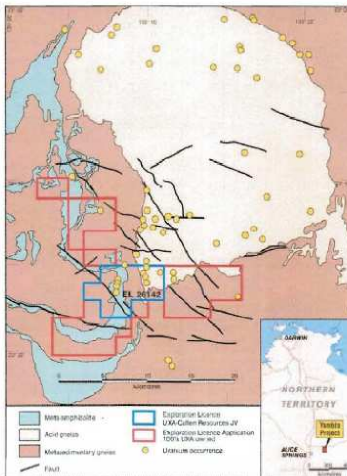
Figure 15. Location of Yambula EL 26142 Figure from UXA announcement to ASX of 14 April 2010
