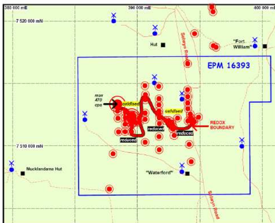
Figure 9. Reconnaissance drilling by PNC Exploration (Australia) Pty Ltd Compiled by D G Jones from McKay (1983) and Dunn (1983)
