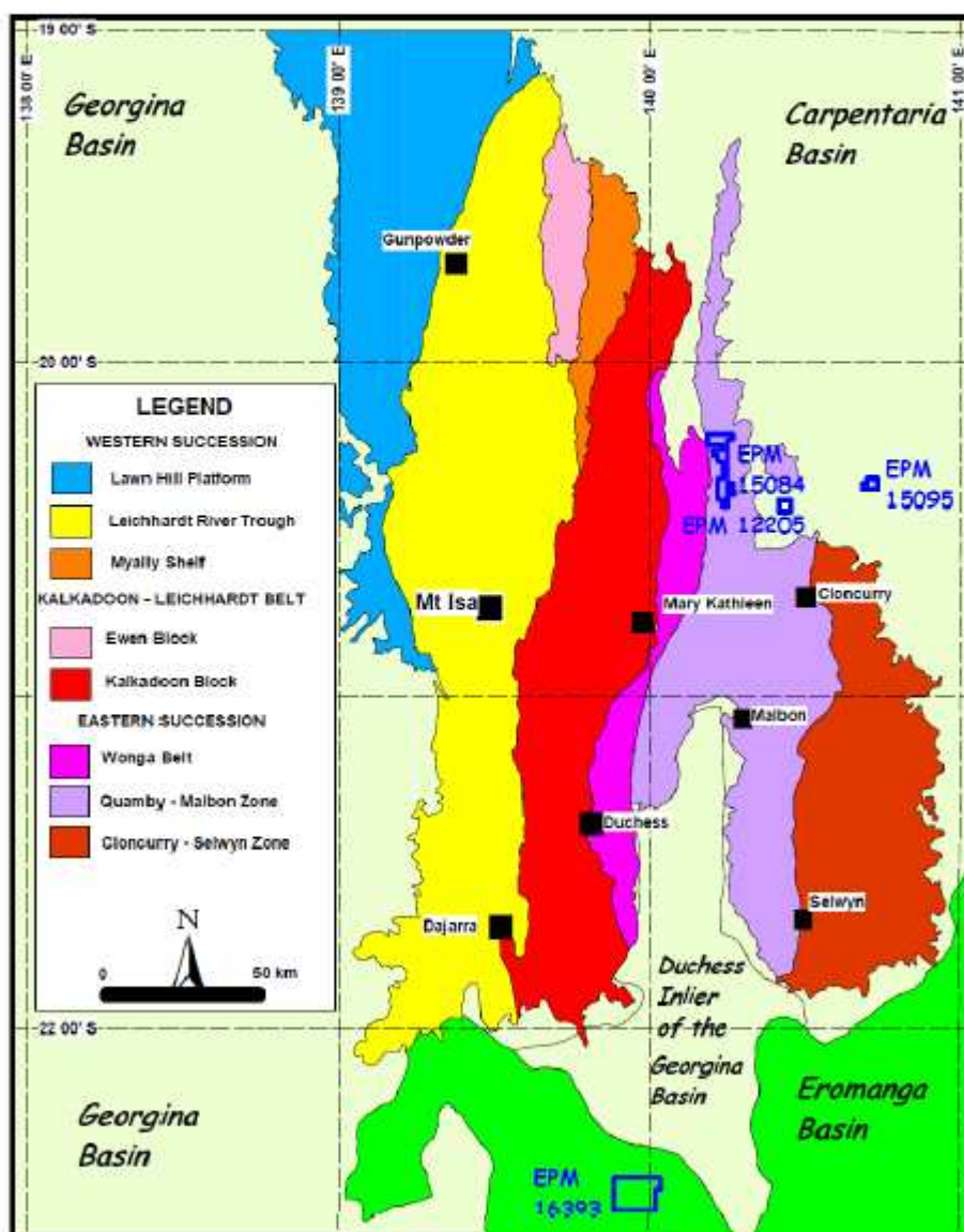
Figure 5. Regional geology, Mt Isa Inlier Figure compiled by D G Jones
