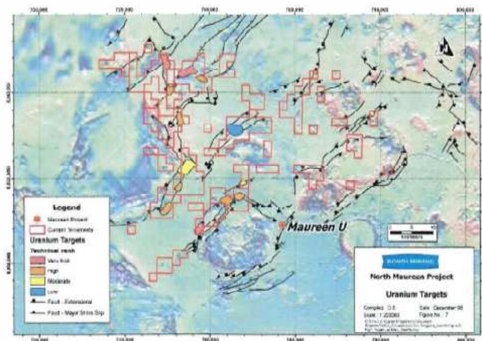
Figure 16. North Maureen targets superimposed on magnetic image Figure from Bondi ASX announcement 23 February 2010
