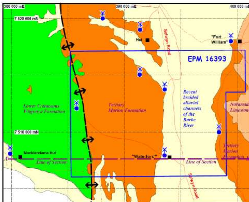
Figure 7. Surface geology, EPM 16393 Compiled by D G Jones from Casey et al (1967)
