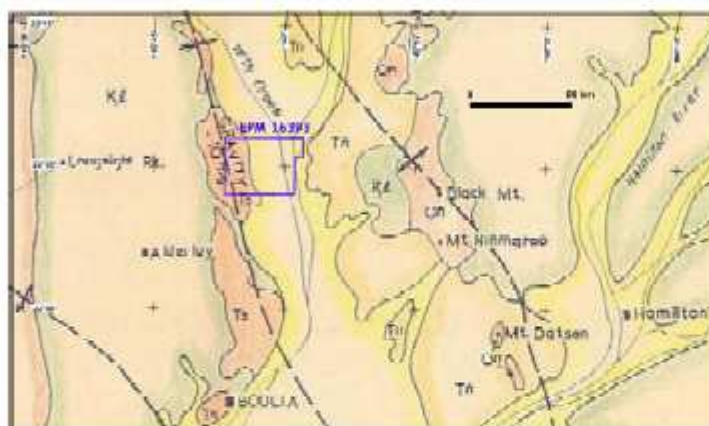
Figure 4. BMR map 1958 Figure from Laing (1958)
