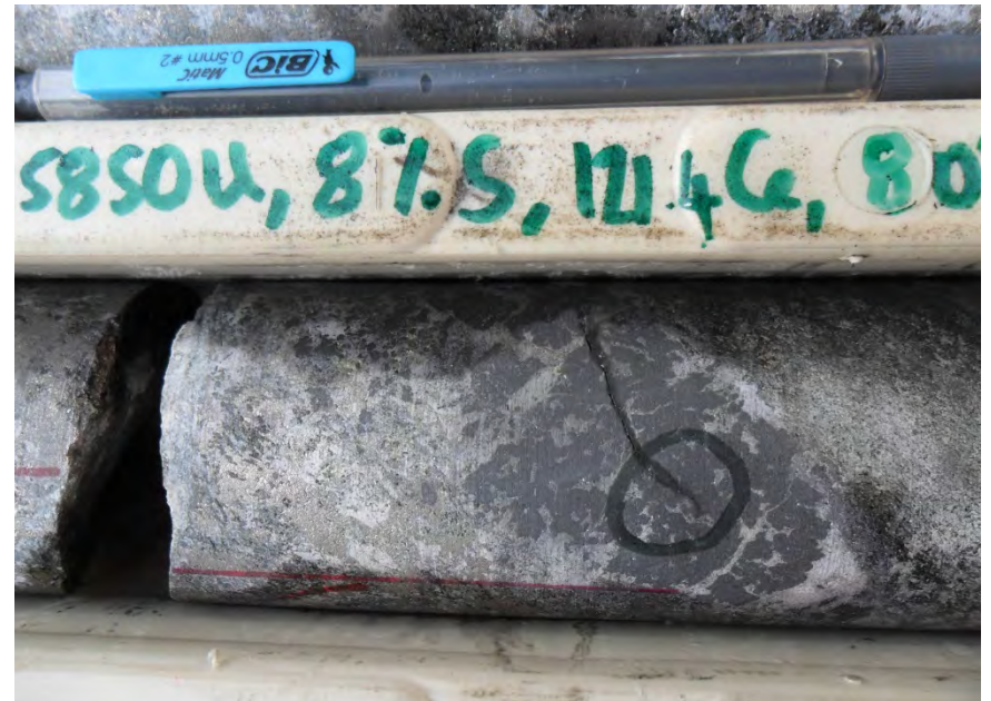
MKED009 – 508m – Massive uraninite (“pitchblende”) +/- allanite PXRF – 5,850 ppm U. (6.9 kg/t U_3O_8 )
