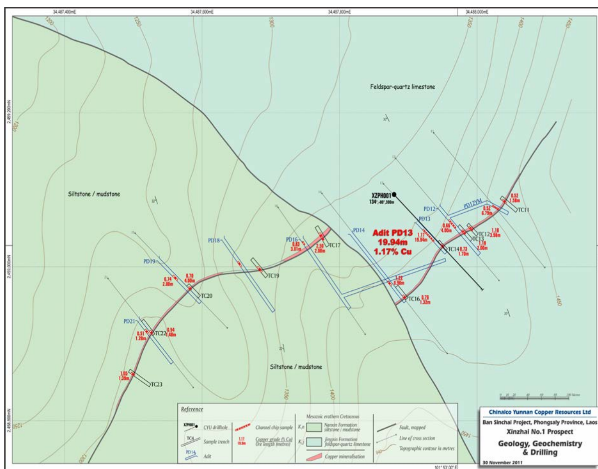
Figure 2. Hole XZPH001 is to test the dipping extension of known mineralisation defined by trenches and adits
