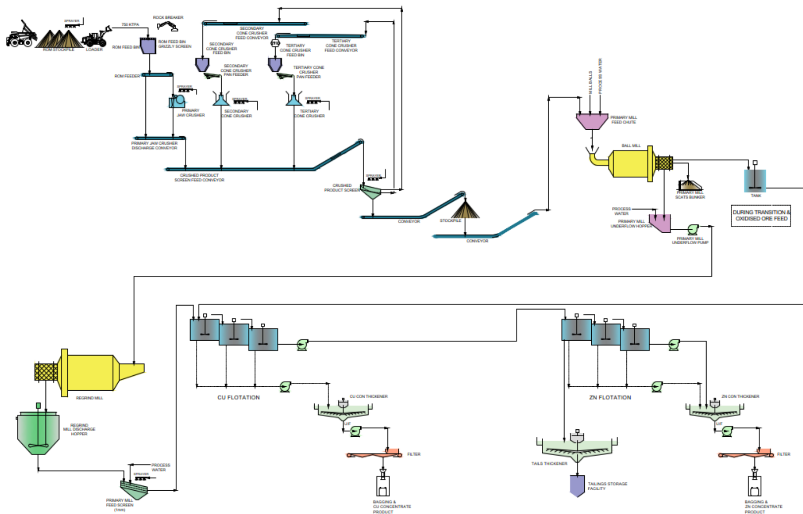
Figure 8-1: Proposed Koongie Park Processing Flowsheet Block Flow Diagram
