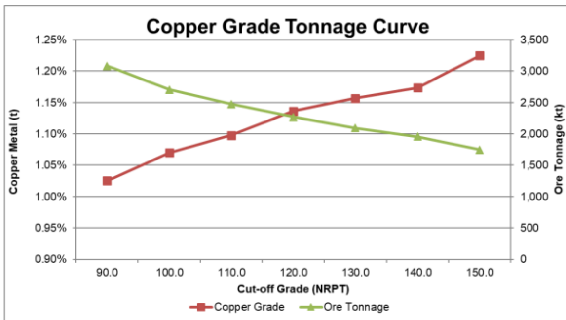
Figure 6-10: Copper Grade Tonnage Curve
