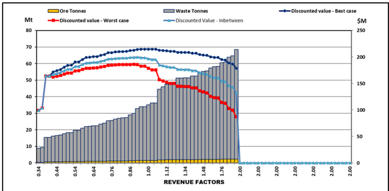
Figure 6-2: Discounted Best-Case Mining Scenario
