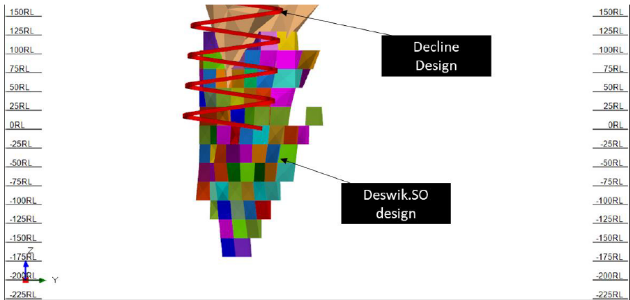
Figure 6-13: Underground Design looking from East
