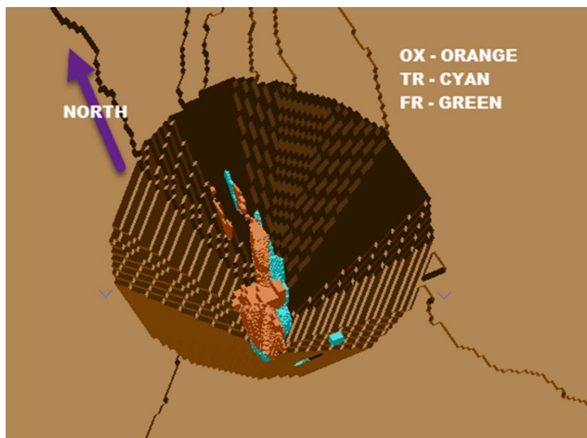
Figure 6-4: Shell 20 with the Reblocked Model
