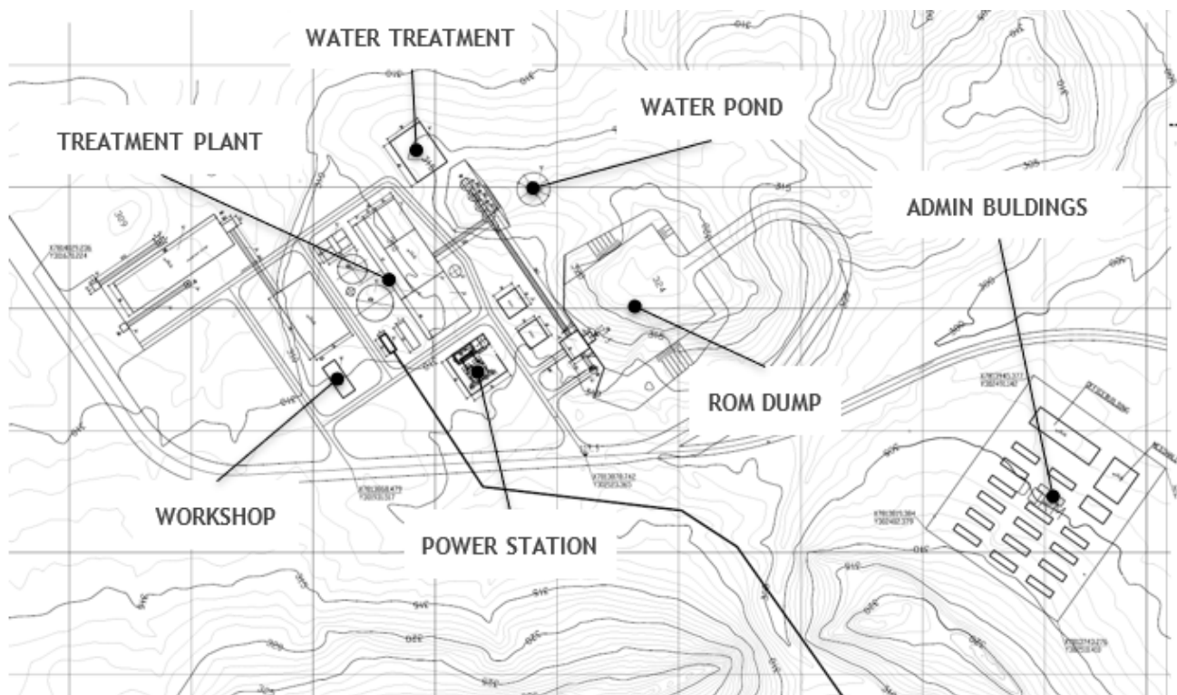
Figure 9-1: Site Layout
