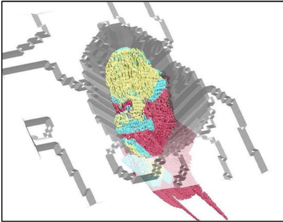
Figure 6-9: Mt Angelo North Pit Shell Pit 9
