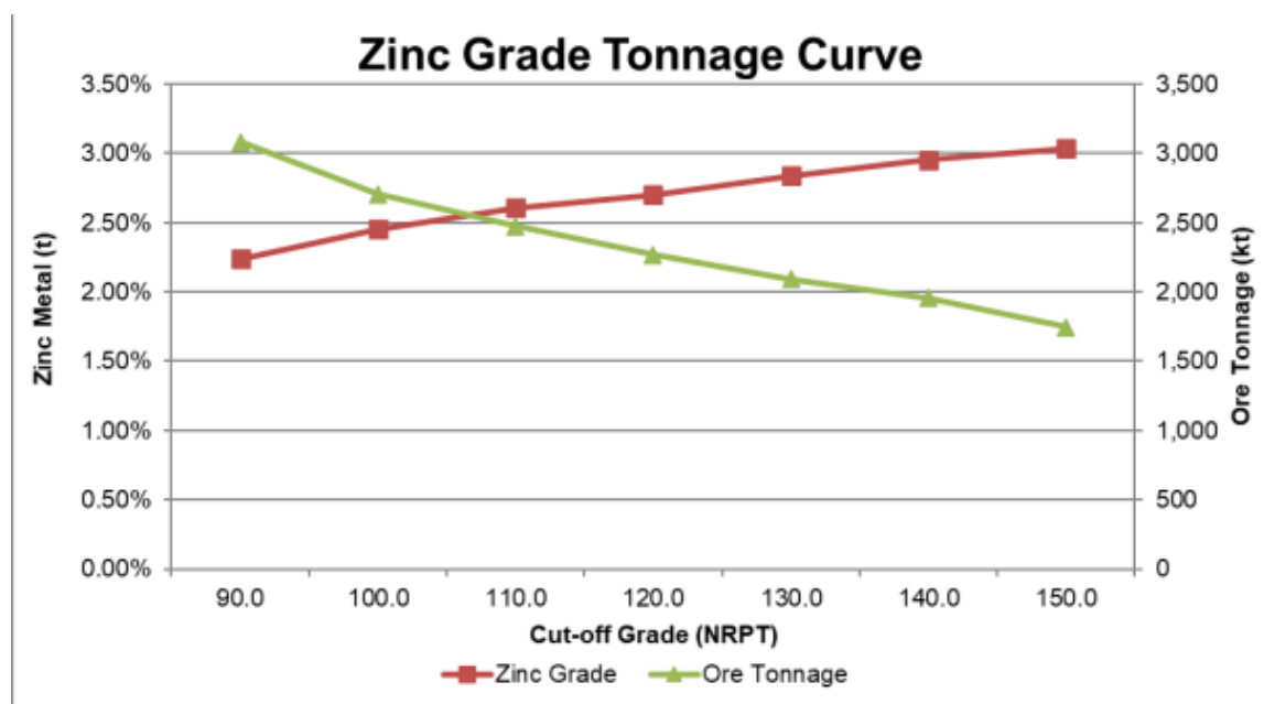
Figure 6-11: Zinc Grade Tonnage Curve
