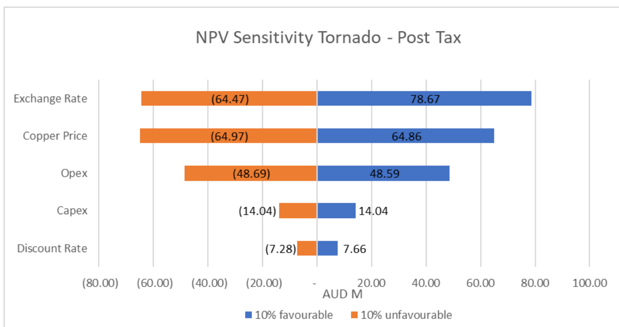
Figure 14-3: Tornado Chart Sensitivity Analysis
