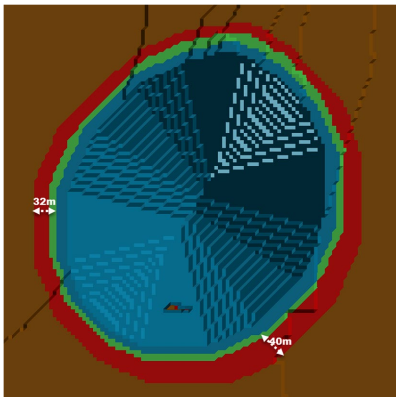
Figure 6-3: Plan View of Pit Shell 20
