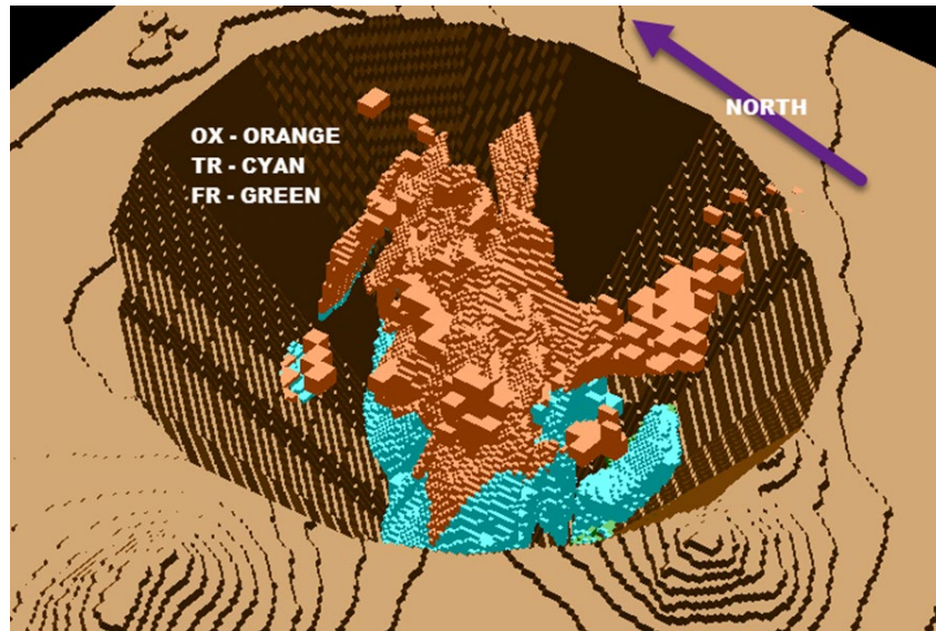
Figure 6-8: Shell 17 with the Reblocked Model
