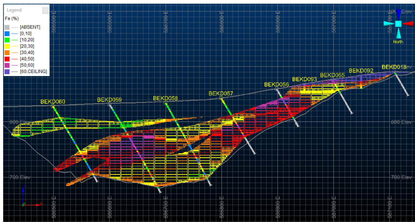
Figure 4. A newly defined “Green Steel Resource” in Bekisopa’s southern zone which graded 45.3% Fe could deliver a 68.7% iron ore concentrate for use in a Direct Reduced-Electric Arc Furnace.
