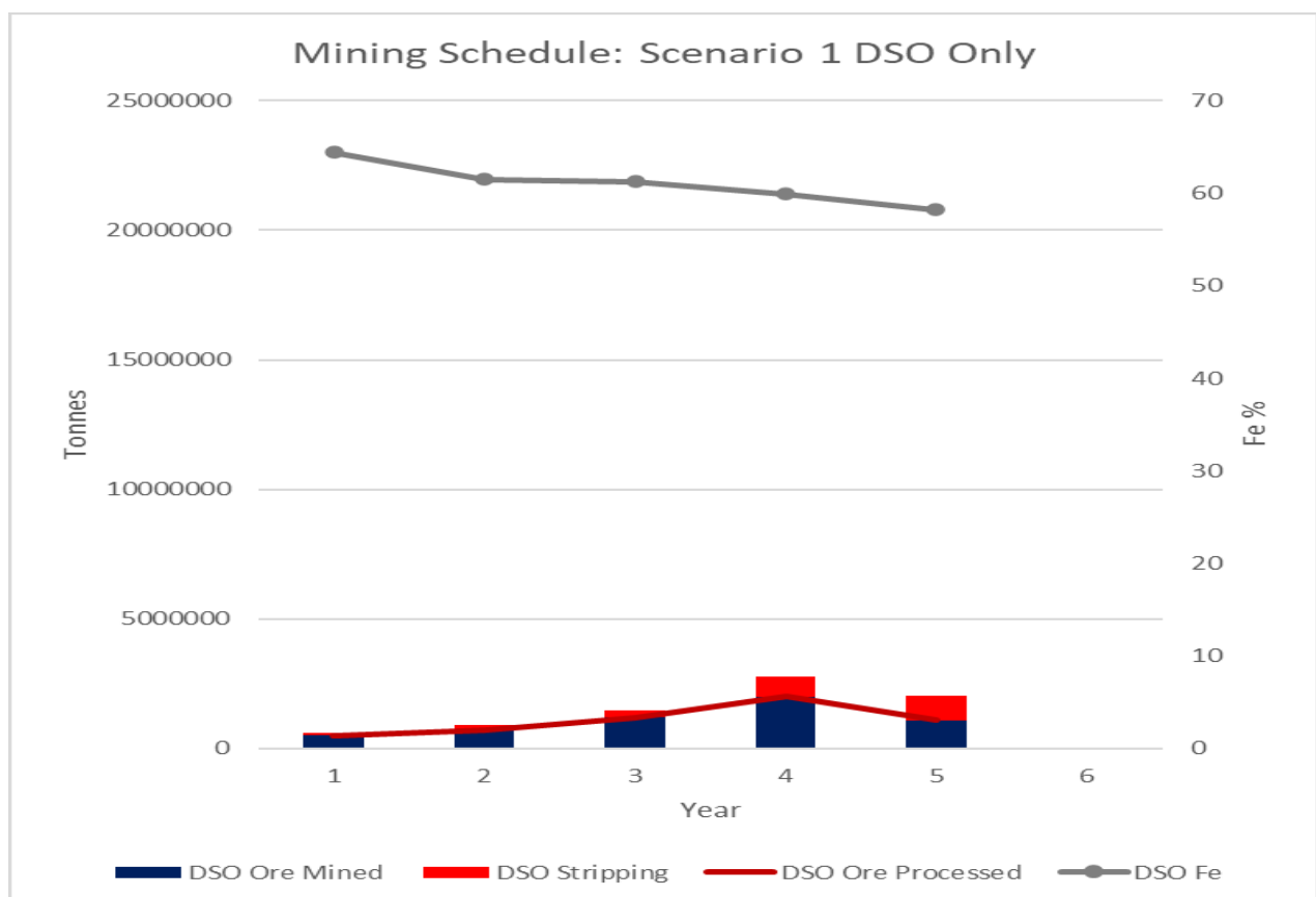
Figure 12a. ‘Low CAPEX Case’ DSO mining schedule.
