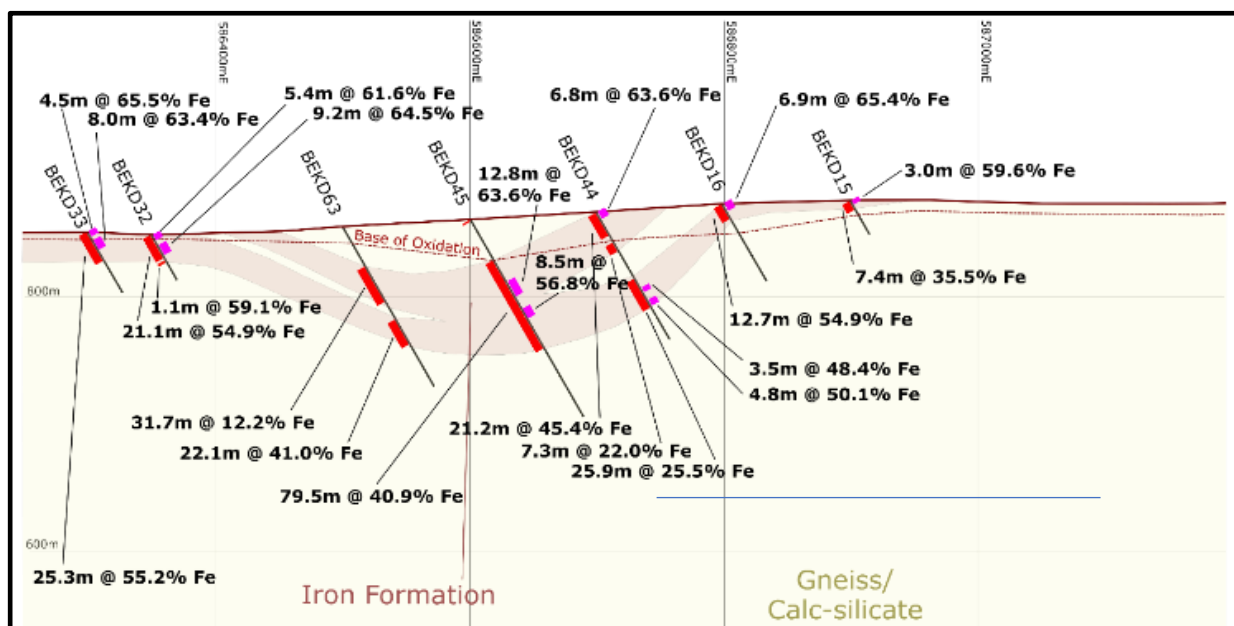
Figure 8a. Bekisopa southern zone cross section 7,608,000N, showing high-grade iron ore in the weathered zone, 59 to 65% Fe, and continuous iron ore mineralisation across strike down to ~140m at grades of ~40% Fe.
