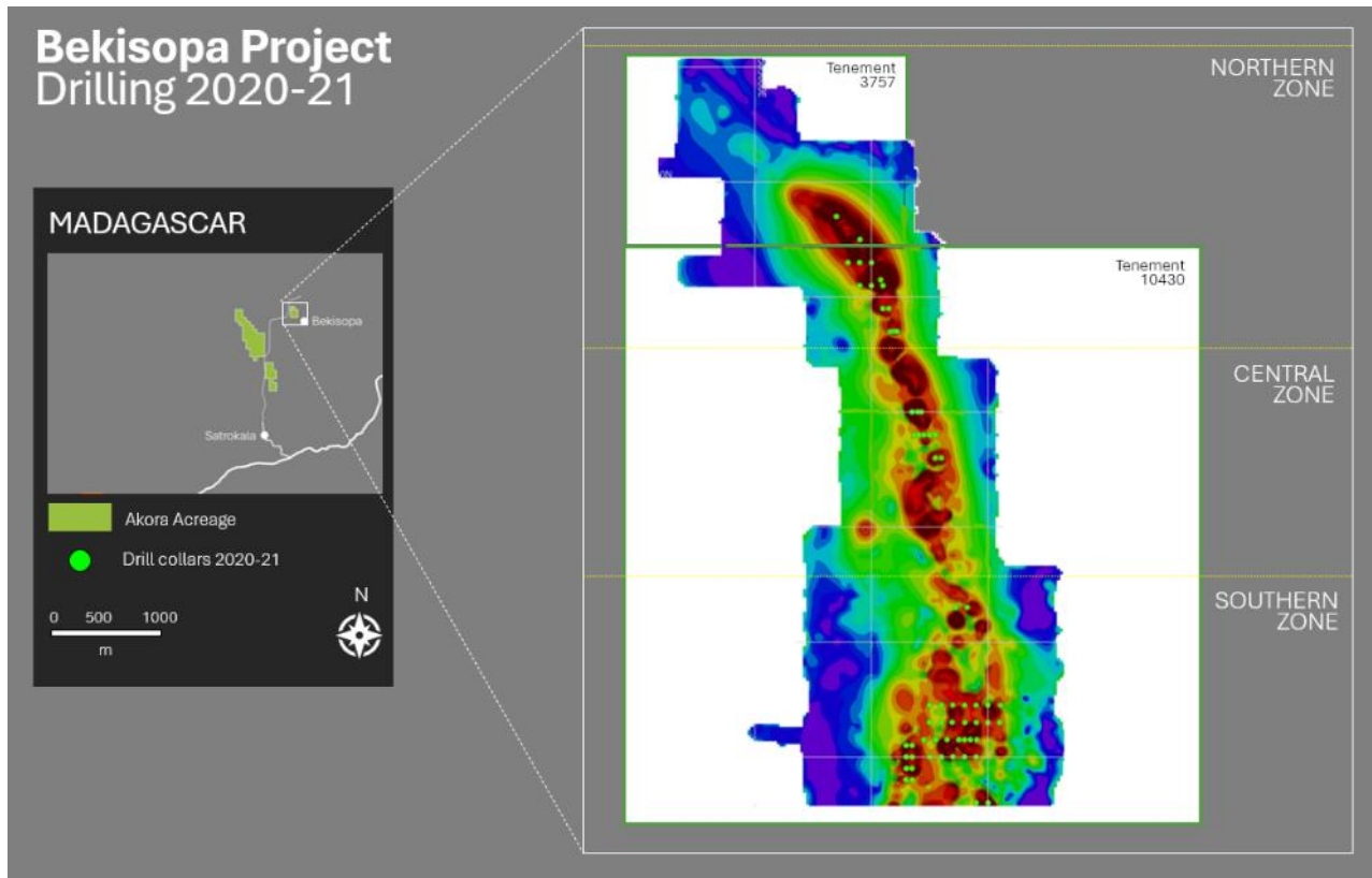
Figure 3. A 194.7Mt maiden JORC Inferred Mineral Resource Estimate (MRE) grading 32% Fe was defined at Bekisopa in April 2022 within just 30% of the 6km mineralised strike length.
