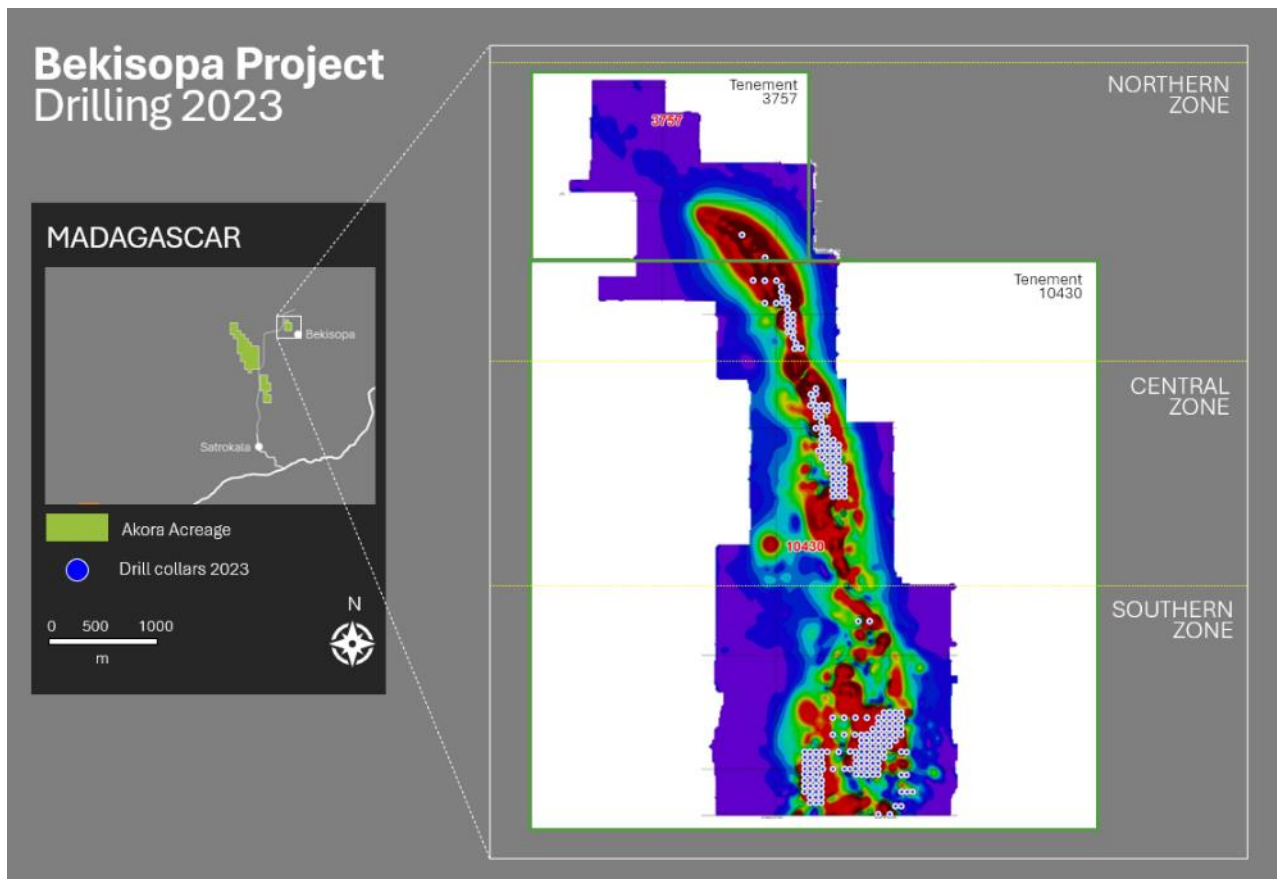
Figure 10. The Bekisopa magnetic anomaly, with all 250 drill holes marked, showing that drilling to date has only covered 40% of the known 6km strike length, potentially offering more DSO tonnes with further drilling.
