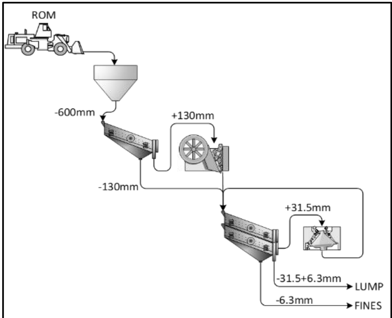
Figure 13. Block Flow Diagram of the Typical Fixed Plant Circuit for DSO Material
