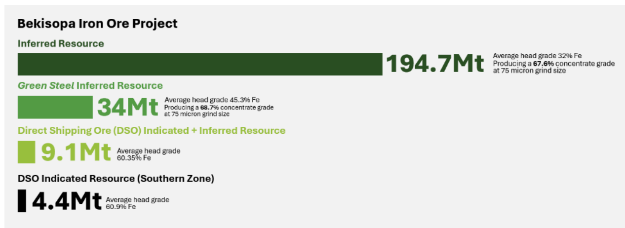
Figure 5. Bekisopa JORC Resource
