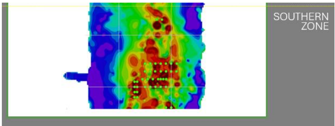
Figure 4. In the project's southern zone, 4.4Mt of Indicated DSO tonnes have been defined according to JORC specifications within the overall total project resource. The Scoping Study prepared by WAI was based on the DSO resource estimated in the July 2023 WAI MRE report.
