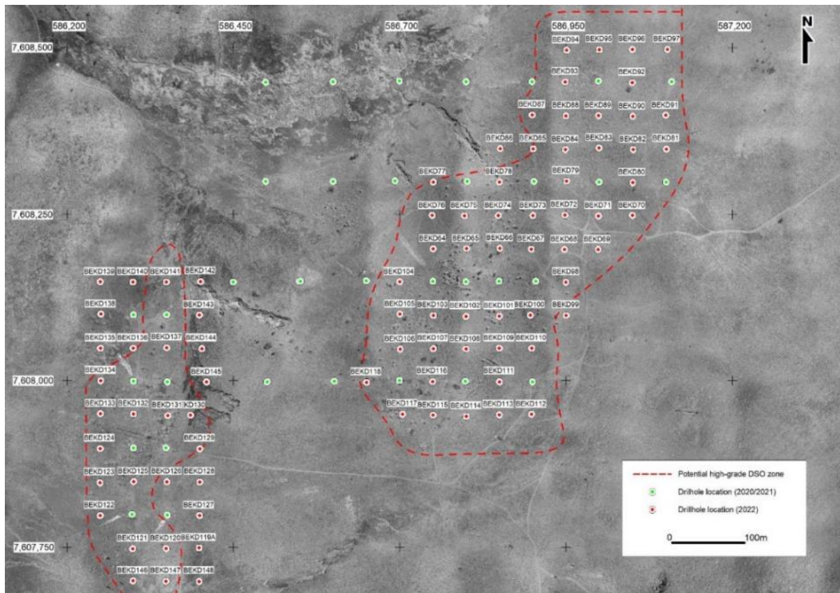
Figure 9. Bekisopa 2022 DSO infill drill hole locations on the eastern and western sides of the Southern Zone from which determined Indicated DSO Resource of 4.4Mt at 61% Fe.
