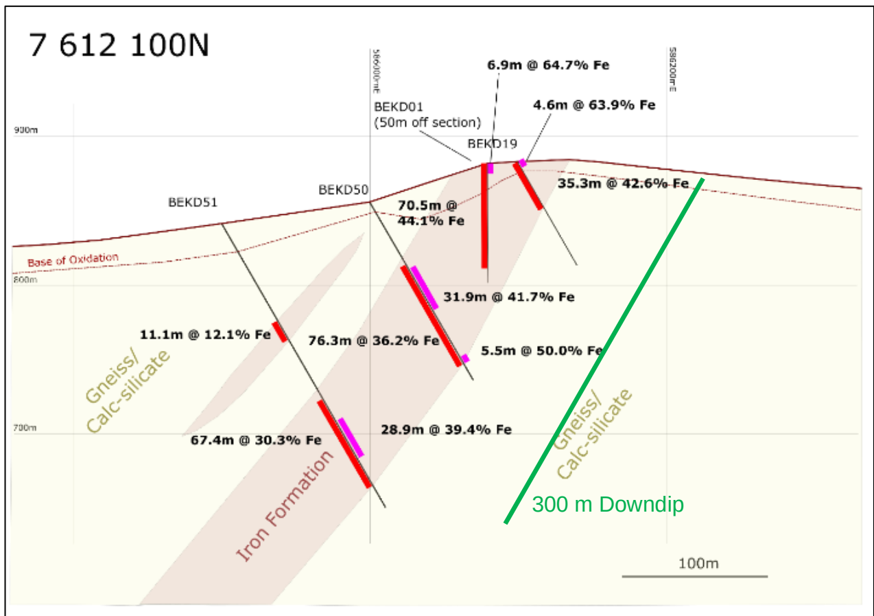
Figure 7a. Bekisopa northern zone cross section 7,612,100N, showing high-grade iron ore in the weathered zone, ~64% Fe, and continuous iron ore mineralisation down dip to +300m at grades of ~35% Fe.
