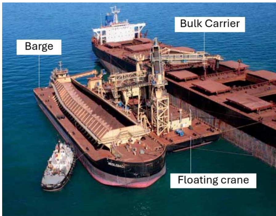
Figure 18. Floating crane transferring from a barge onto a bulk carrier.
