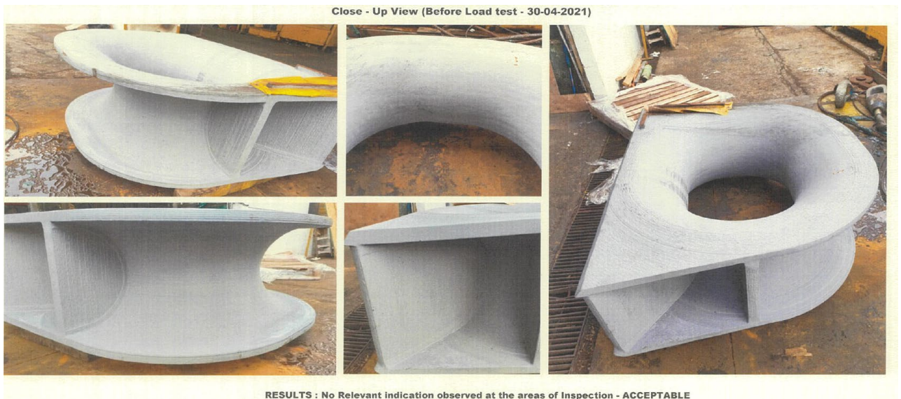
Deck mounted type Panama Chock (SWL150Ton) produced during the additive manufacturing project.
