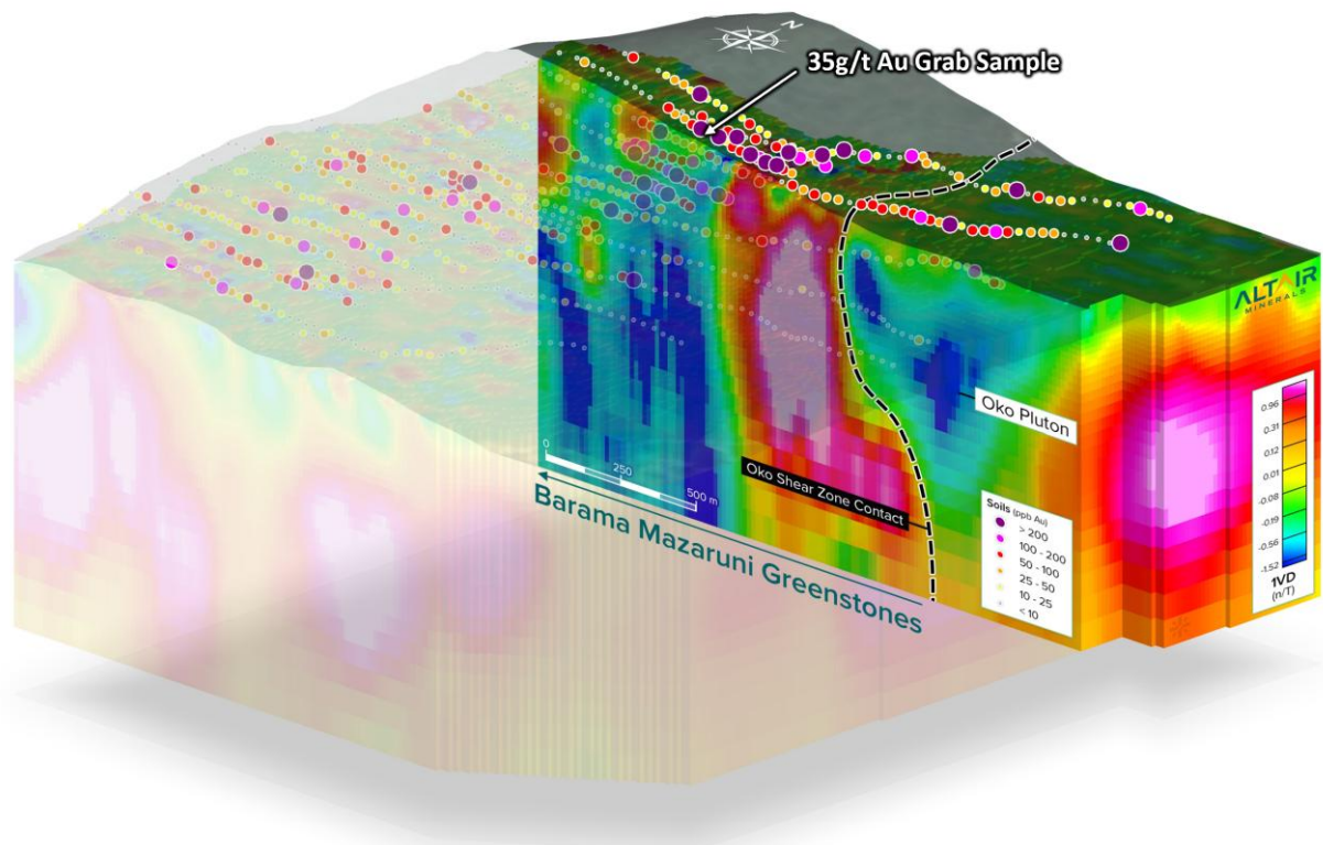
Figure 1: 3D view of magnetic inversion at SOKO, cut at 695200N, with soil samples to date overlaid. 24
