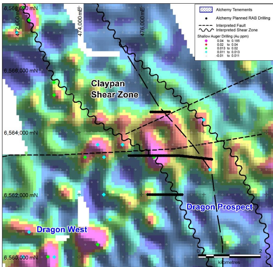
Figure 4: Dragon Prospect planned RAB drill lines (black dots), previous auger drilling, and interpreted Claypan Shear Zone over gold in auger drilling image.
