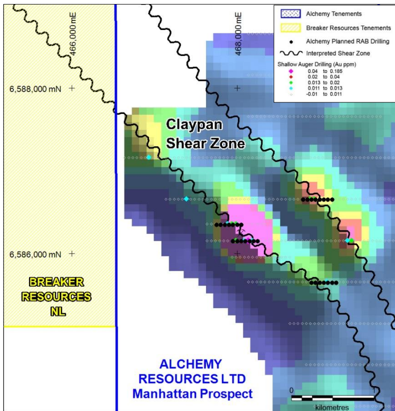
Figure 3: Manhattan Prospect planned RAB drill lines (black dots), previous auger drilling, and interpreted Claypan Shear Zone over gold in auger drilling image.
