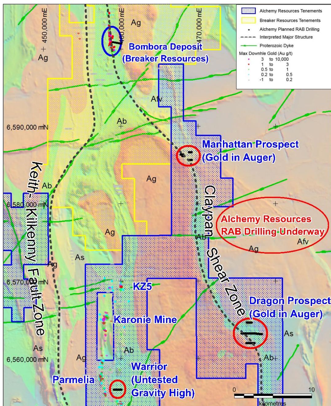
Figure 2: Karonie Project planned RAB drill lines (within red circles), previous drilling maximum downhole gold, Alchemy and Breaker Resources tenement outlines, and relevant prospects over regional transparent Govt. geology over aeromagnetic image.
