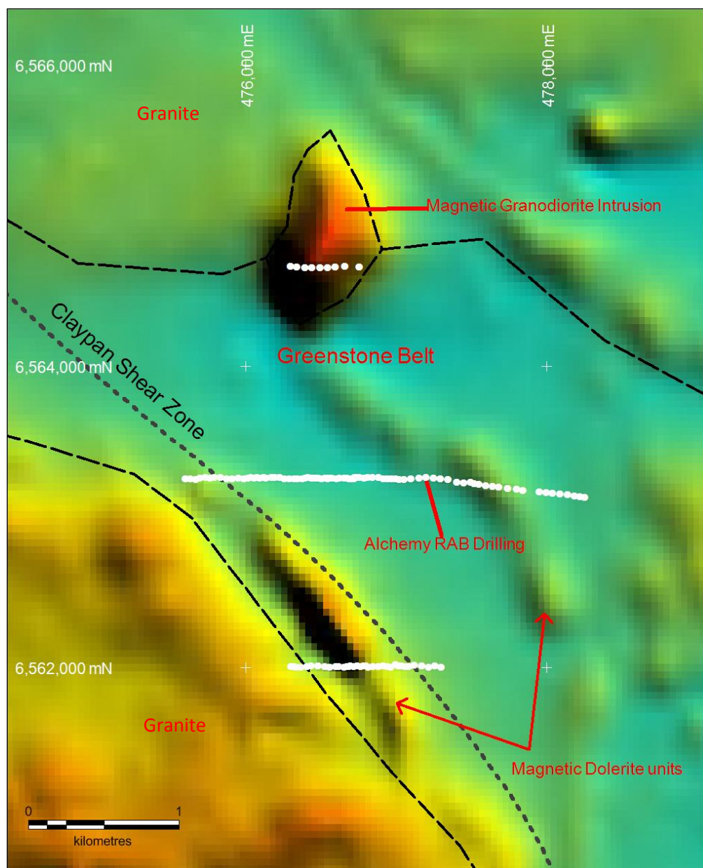
Figure 2: Dragon Prospect completed RAB drill lines (white circles), and interpreted geological features over aeromagnetic image.
