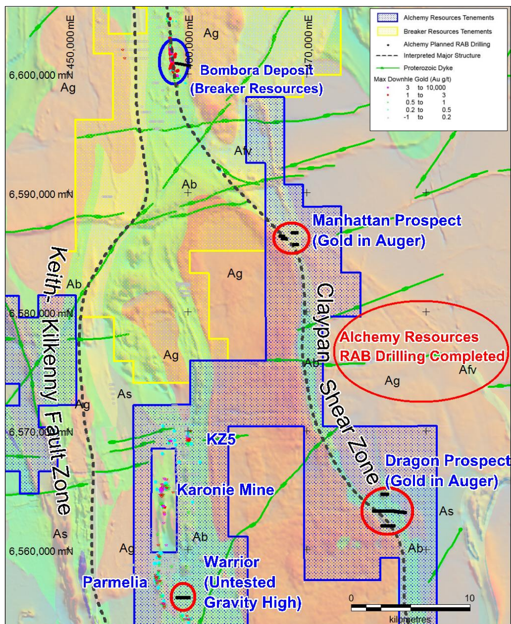
Figure 3: Karonie Project completed RAB drill lines (within red circles), previous drilling maximum downhole gold, Alchemy and Breaker Resources tenement outlines, and relevant prospects over regional transparent Govt. geology over aeromagnetic image.
