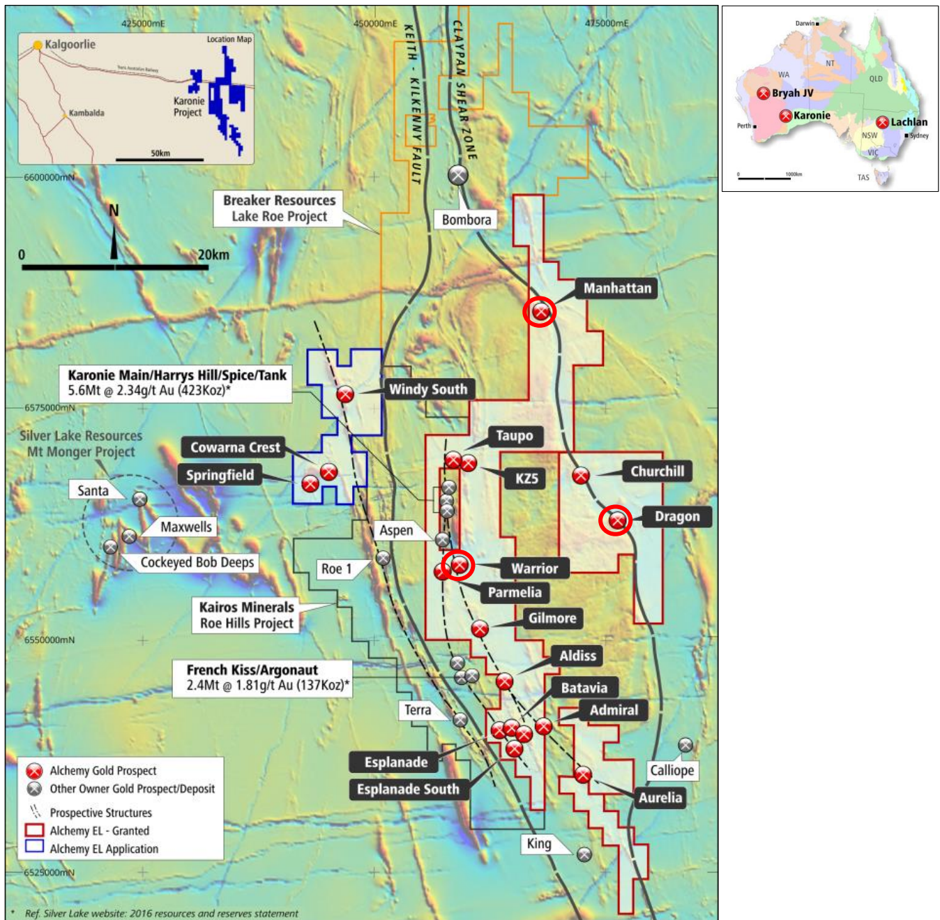
Figure 1: Karonie Project tenements, major deposits, prospects, RAB drilling prospects (red circles) and interpreted major structures over aeromagnetic image
