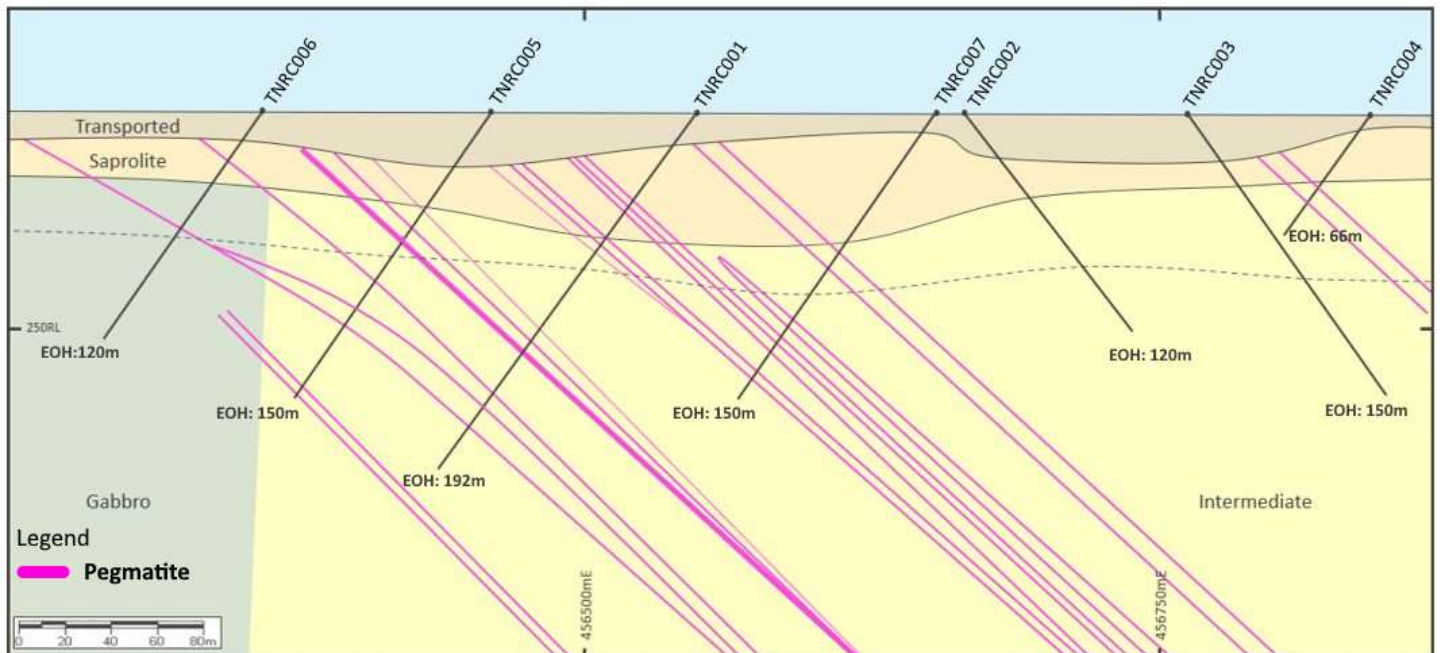
Figure 2: Taupo North cross section 6571930mN showing pegmatite intercepts
