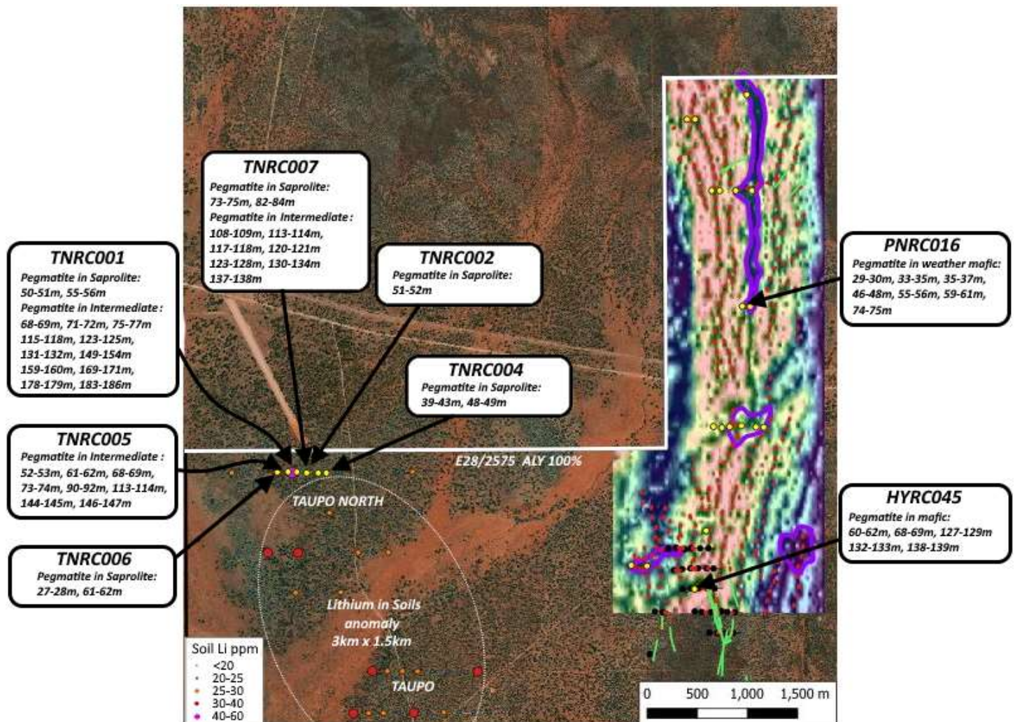
Figure 1: Karonie RC drill program with significant pegmatite intercepts
