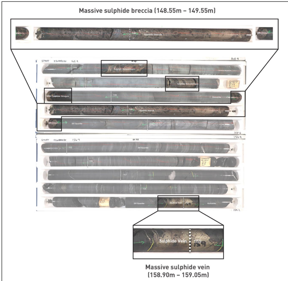
Figure 2: Intersection of nickeliferous sulphides in drillhole 23NDD030, with some massive sulphide intersections highlighted.
