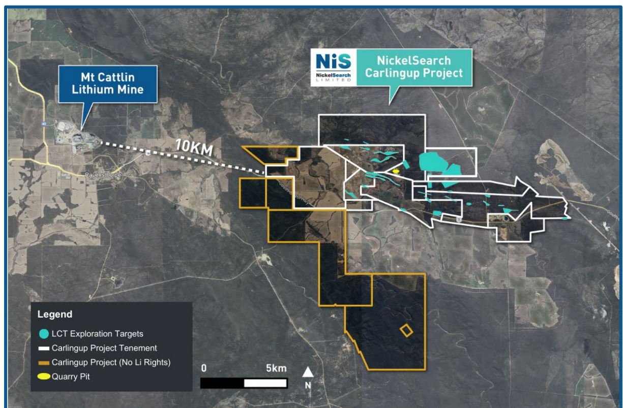
Figure 6: Map of Ravensthorpe area showing Allkem's Mt Cattlin and NIS' Carlingup, with tenements with Lithium rights outlined in white.
