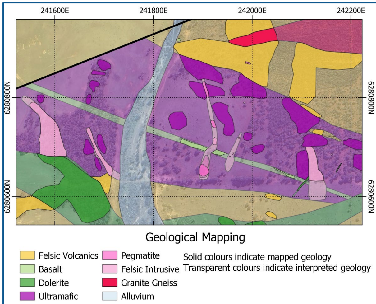
Figure 2: Portion of the geological mapping completed over the southern two high priority lithium areas of interest. Pegmatite and other felsic intrusive rocks were mapped within the area.
