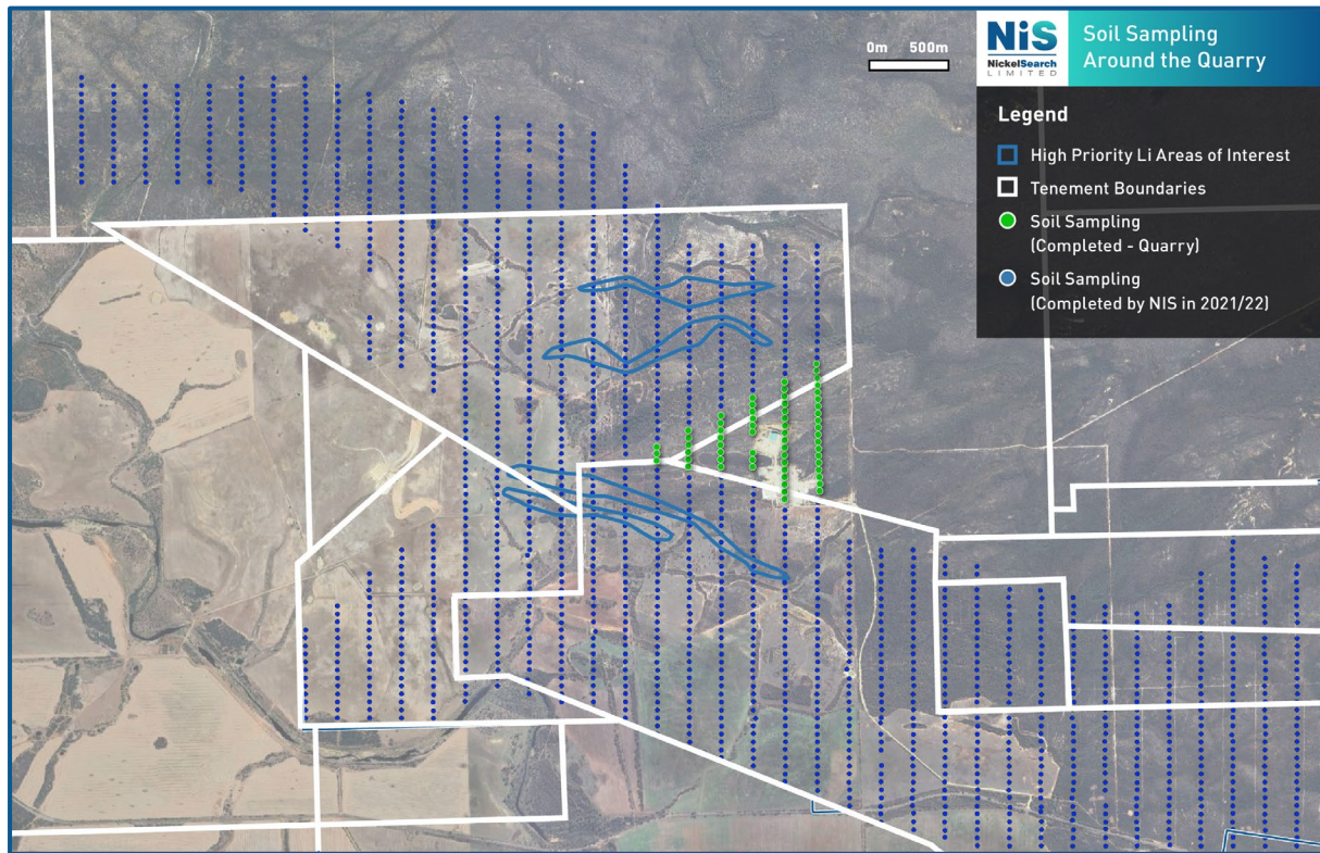
Figure 5: Location of soil sampling completed at the quarry (green dots).
