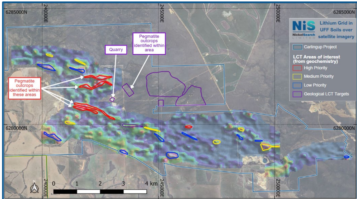
Figure 1: Lithium areas of interest: Ultrafine soil sample Li grid over satellite imagery. Pegmatite outcrops were located within each of the four high priority areas, and within the area north-east of the quarry.
