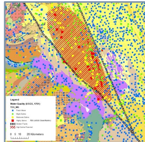
Saline Ground Water
