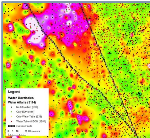
Ground Water Levels
