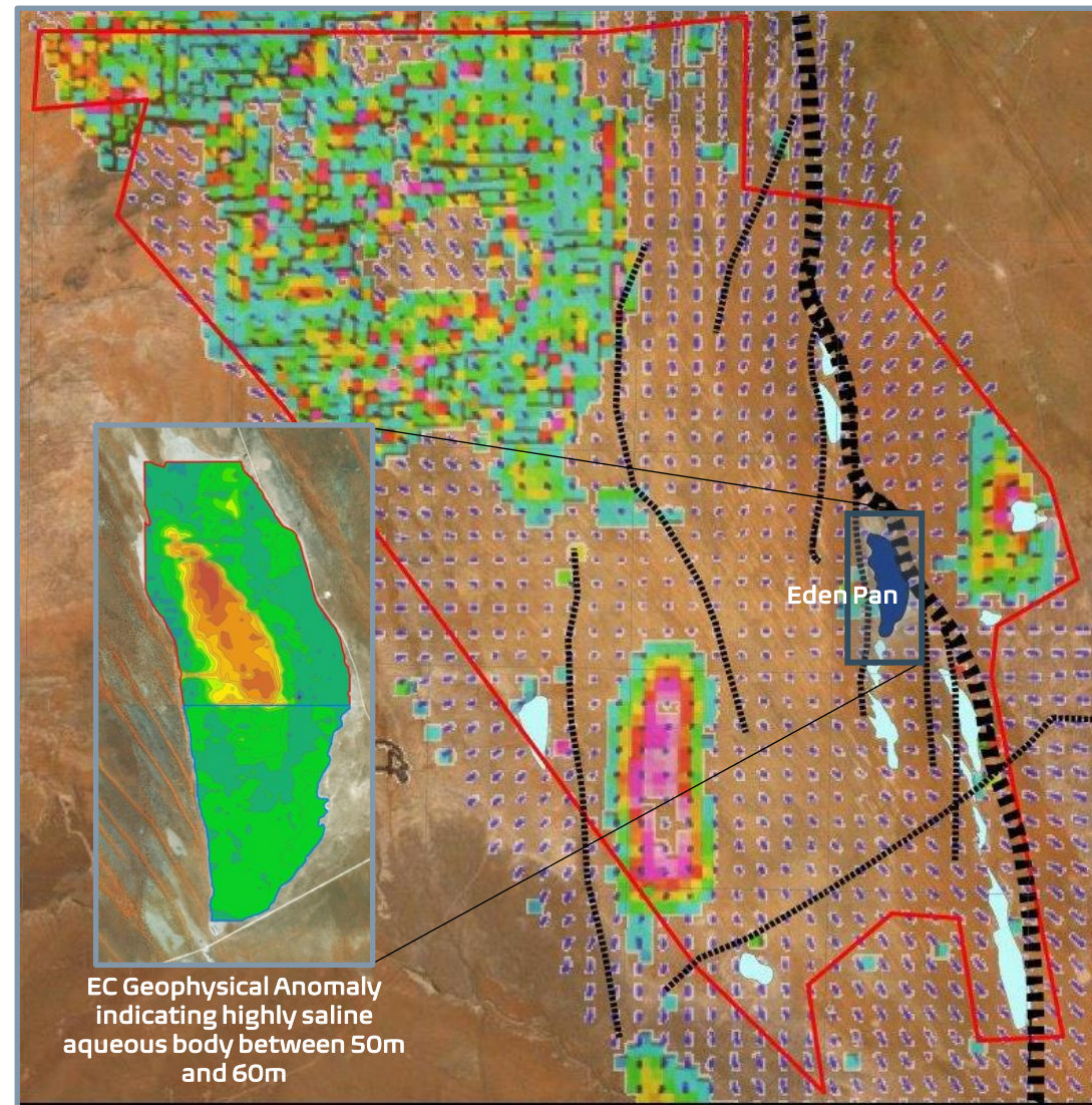
Figure: Schematic model of the Bitterwasser System to aid Arcadia's exploration for lithium-in-clay and lithium-in-brine mineralisation.
