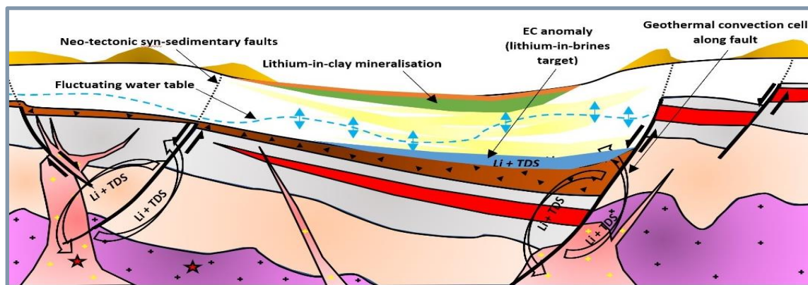
Figure: Schematic model of the Bitterwasser System to aid Arcadia's exploration for lithium-in-clay and lithium-in-brine mineralisation.
