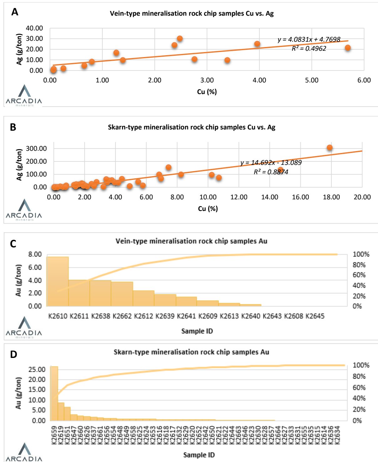
Figure 4 – Plot of Ag vs. Cu for all rock chip samples to date of vein-type mineralisation. B – Plot of Ag vs. Cu for all rock chip samples to date of skarn-type mineralisation. C – Cumulative frequency plot of returned Au contents for all rock chip samples to date of vein-type mineralisation. D – Cumulative frequency plot of returned Au contents for all rock chip samples to date of skarn-type mineralisation.
