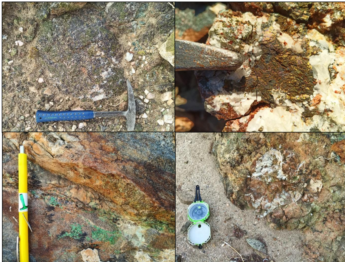
Figure 3: Examples of various outcrops which were rock chip sampled on the Karibib Project to date. A – Outcropping retrograde skarn. B – Various copper sulphides in outcropping skarn. C – Outcropping copper-stained quartz vein in calc-silicate. D – Outcropping skarn in calc-silicate.
