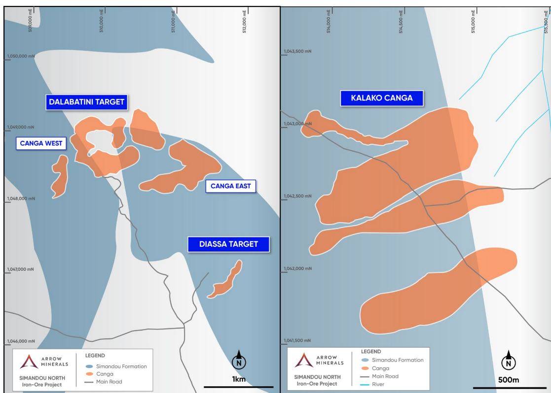
Figure 10: Dalabatini, Diassa and Kalako Canga Targets
