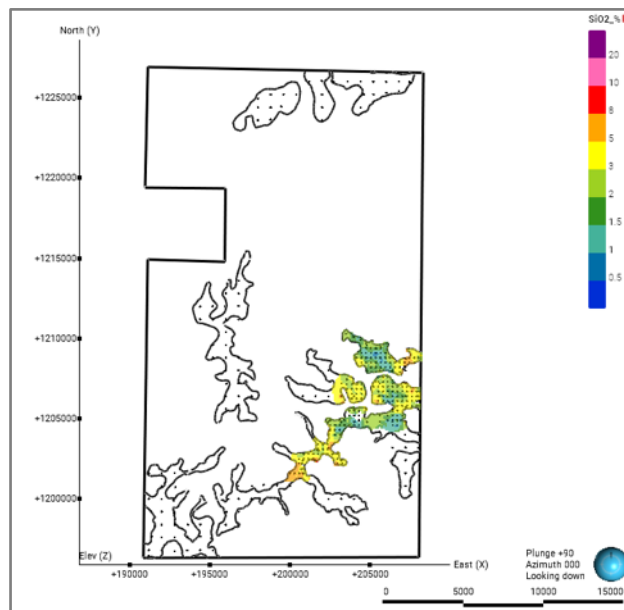
Figure 20. Plan view of the Mineral Resource block model clipped to permit boundary, and thematically coloured by SiO_2 grade (floor to roof) to show grade continuity
