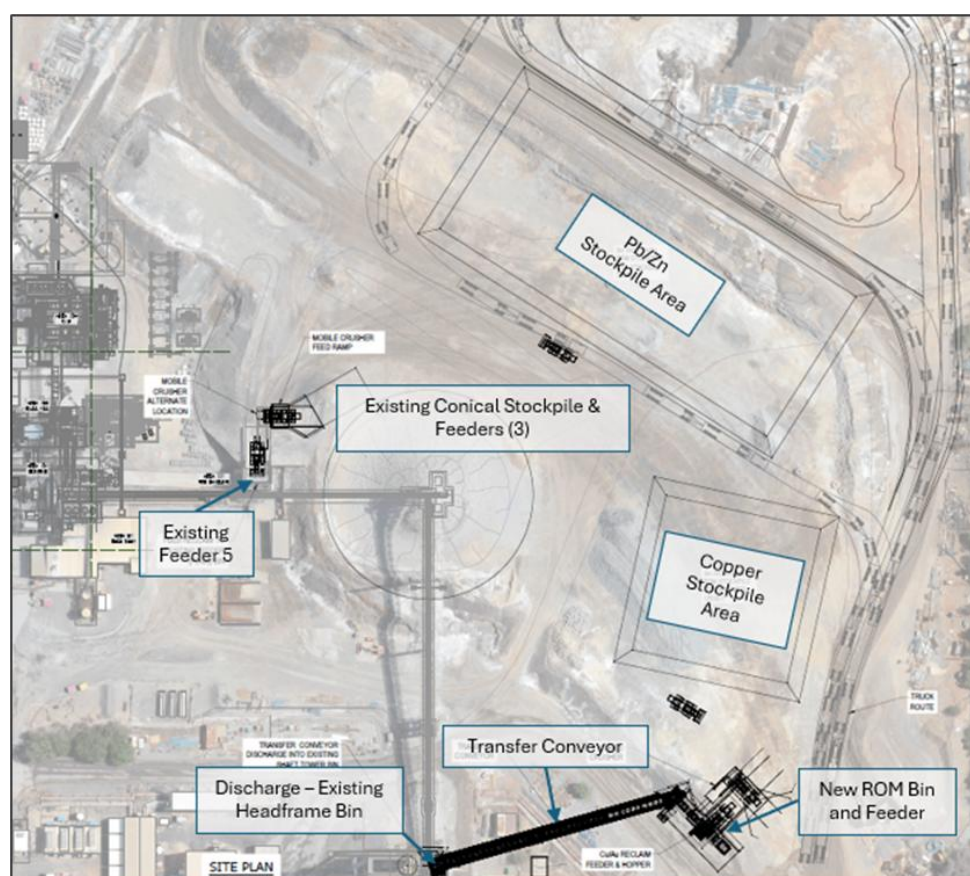
Figure 2: Crushing and materials handling upgrade – general arrangement
