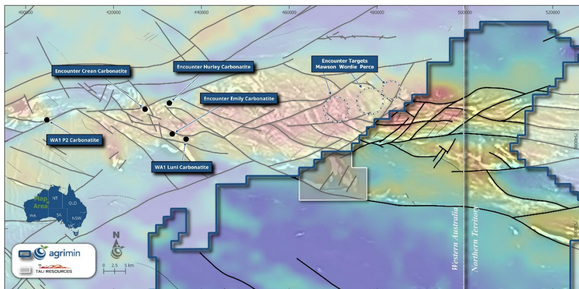
Figure 2. Agrimin's Exploration Tenure with Filtered Gravity over Filtered Magnetics
