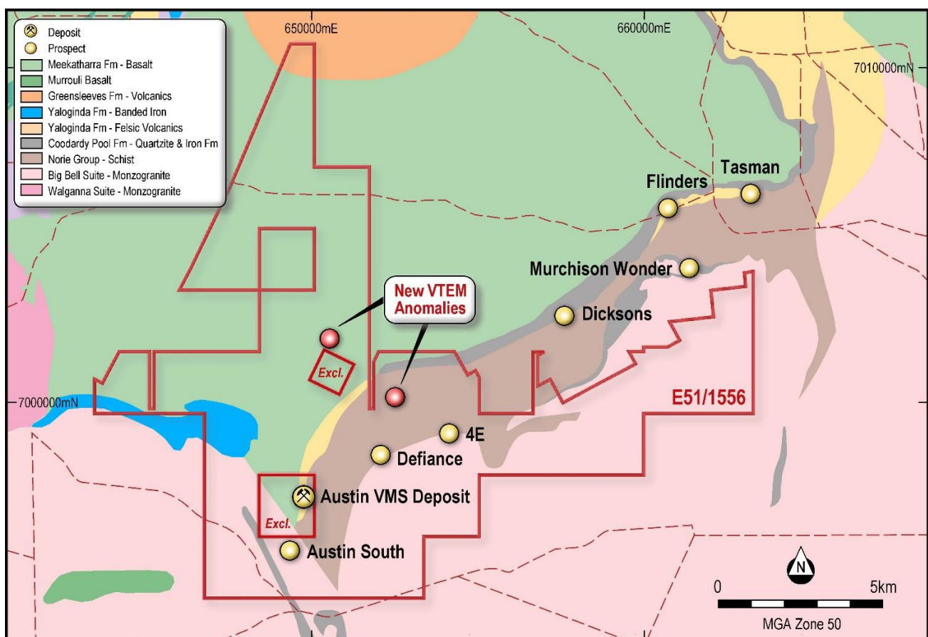
Figure 4. Meekatharra Project – VMS deposits, prospects and VTEM anomalies on GSWA 1:500,000 Geology
