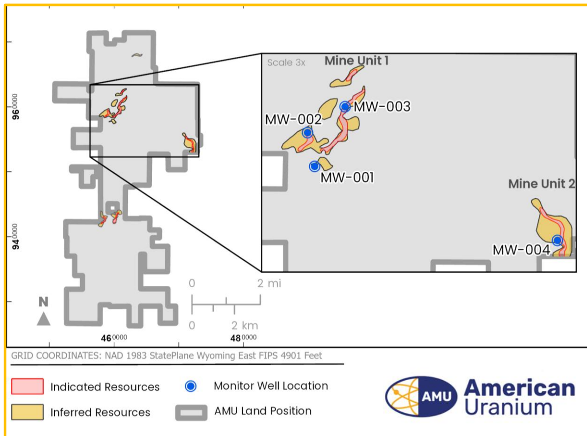
FIGURE 1: LO HERMA MONITOR WELL LOCATION MAP
