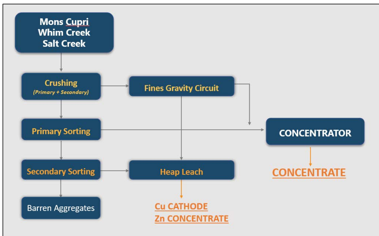
Figure 1: Proposed process flowsheet including two stages of sorting 2
