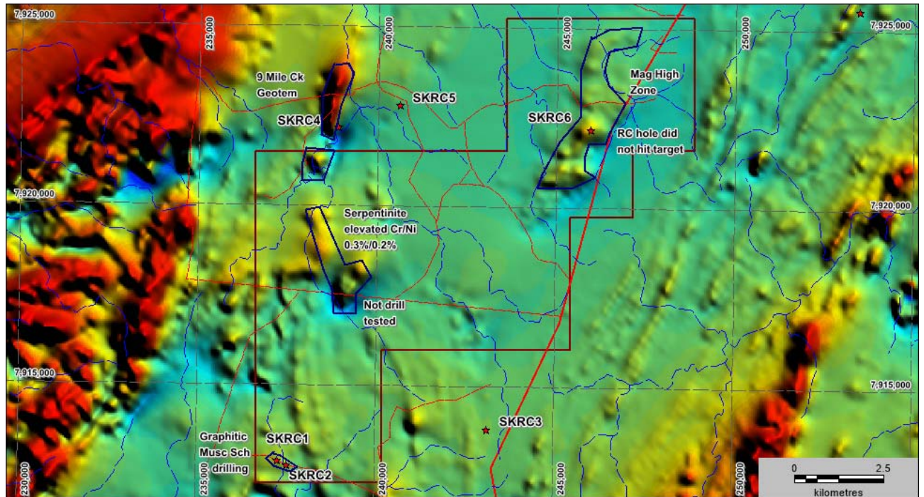
Figure 2 - Greenvale Tenement EL 26813 showing target areas to be visited in the field over TMI Aeromagnetics
