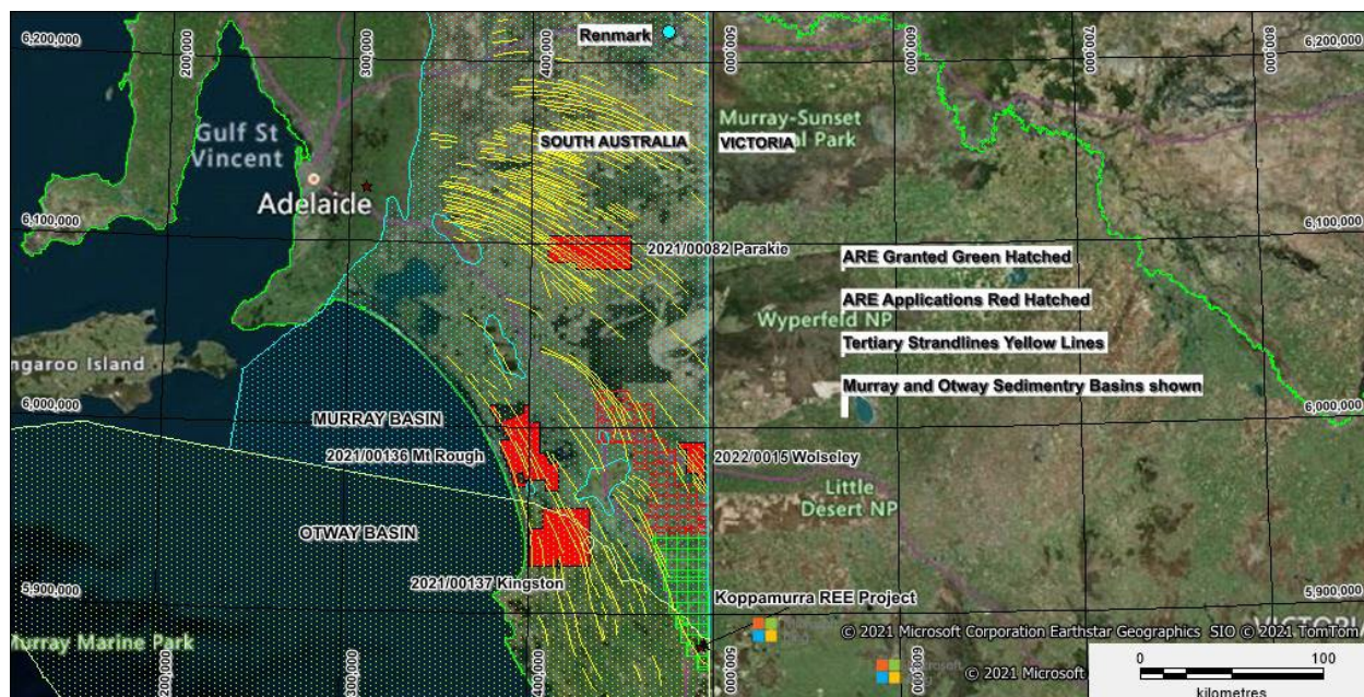
Figure 2: REE Exploration Application Areas within Murray and Otway Basins in SA
