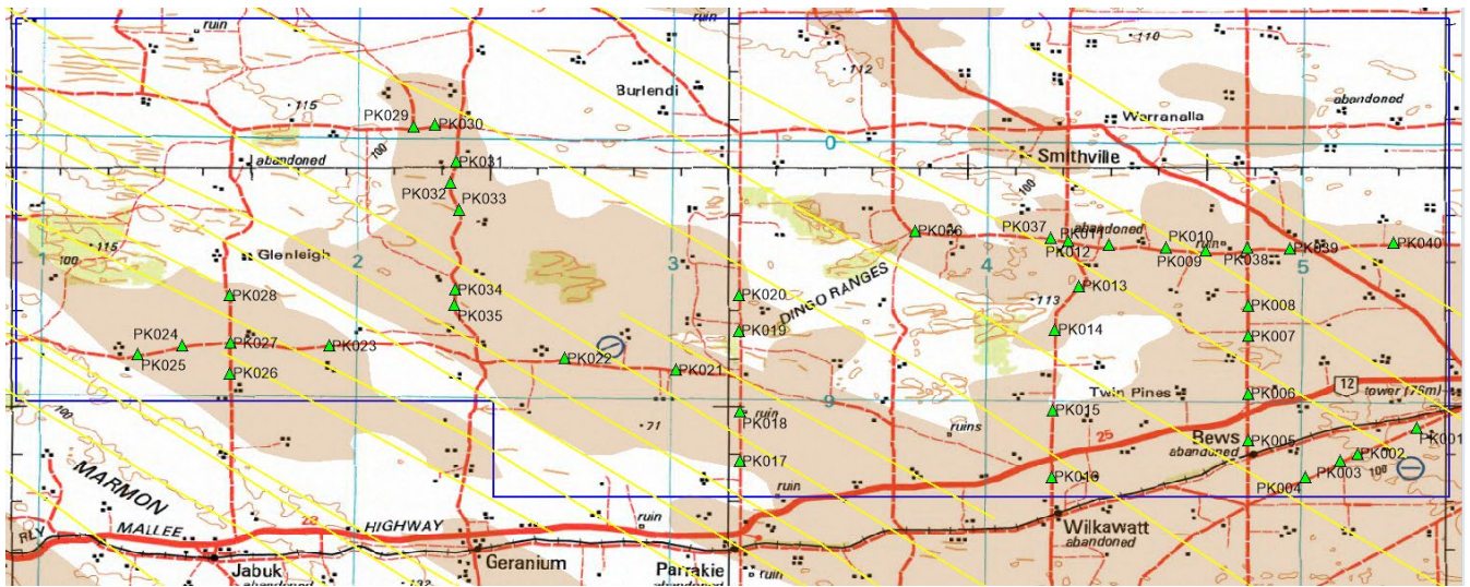
Figure 2: Parrakie aircore drill holes (green diamond) targeting REEs mineralisation within the Loxton/Parilla Sands (brown)
