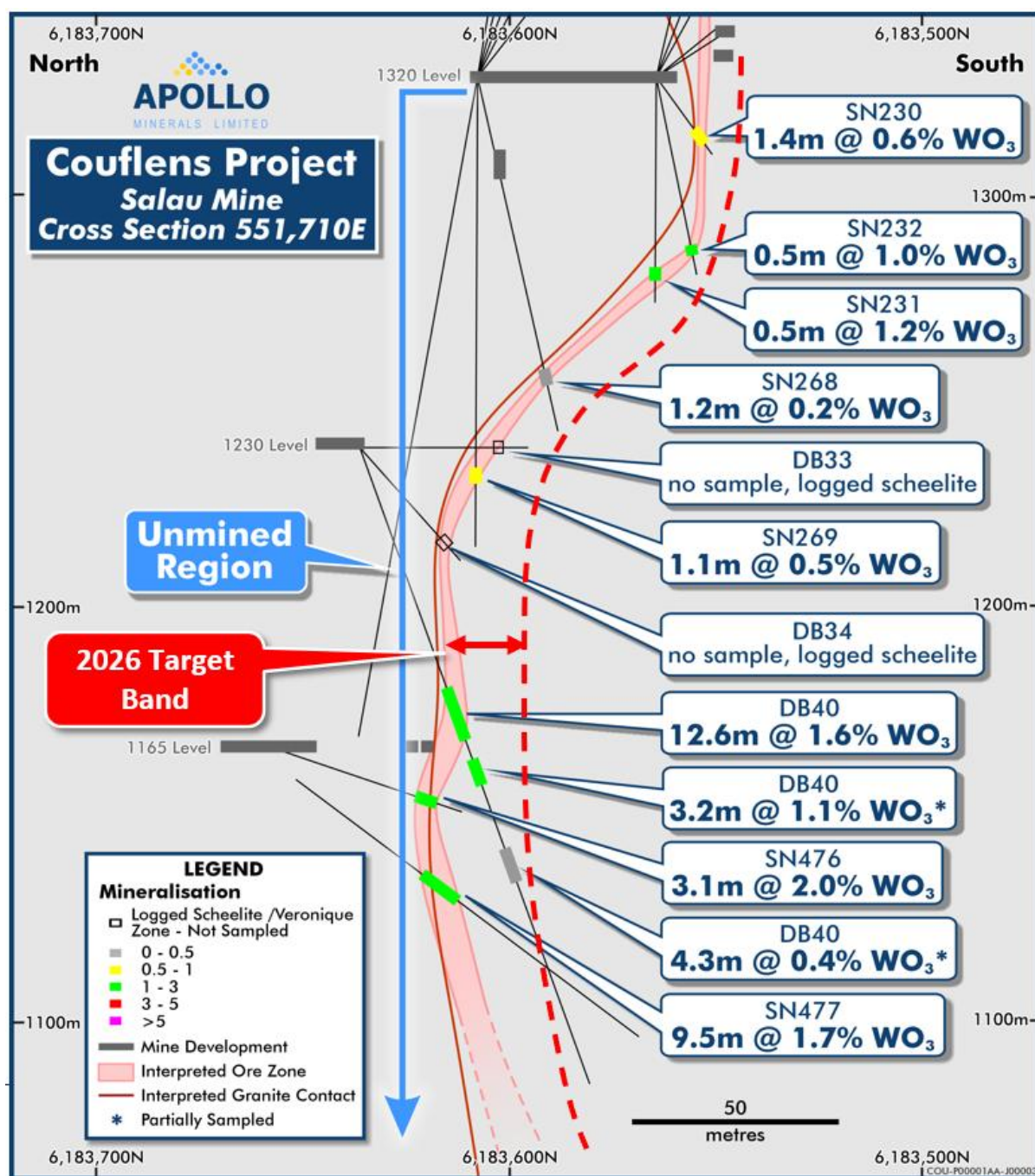
Figure 3: Salau Mine cross section – displaying identified historical drillholes sampled with tungsten assays and intervals with logged scheelite but not sampled. Target band location included for future drill targeting.
