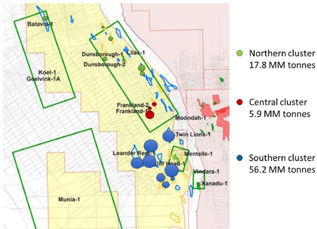
Figure 6 Southern, Central and Northern Clusters of leads and the CCS storage potential associated with each cluster
