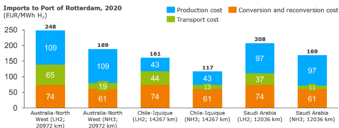
Figure 24 Transportation Cost of Hydrogen and Hydrogen Carriers 26
