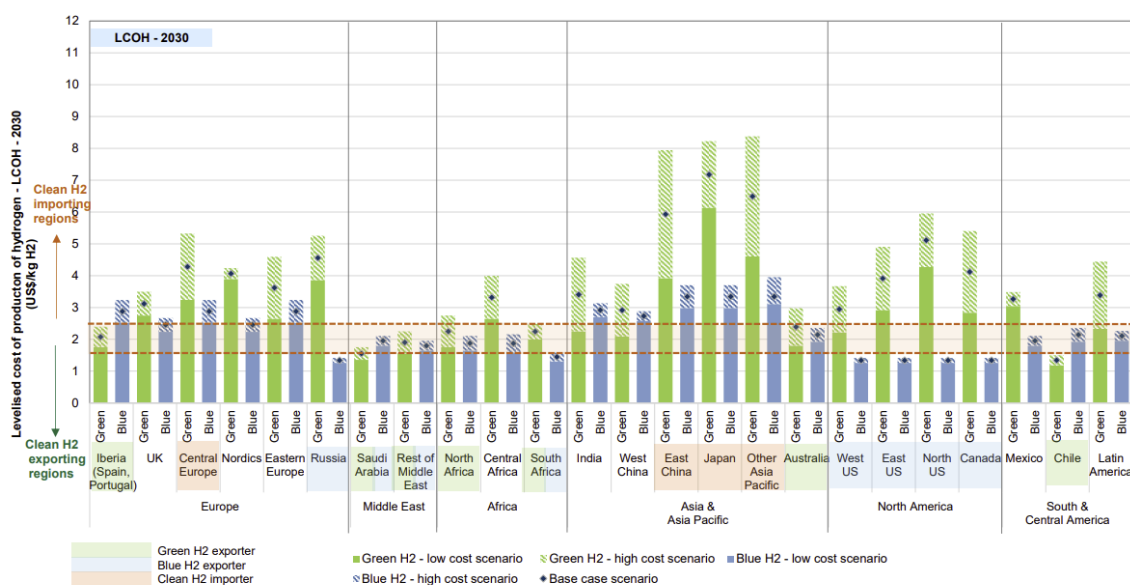
Figure 18 Carbonomics Global Levelized cost of hydrogen in 2030
