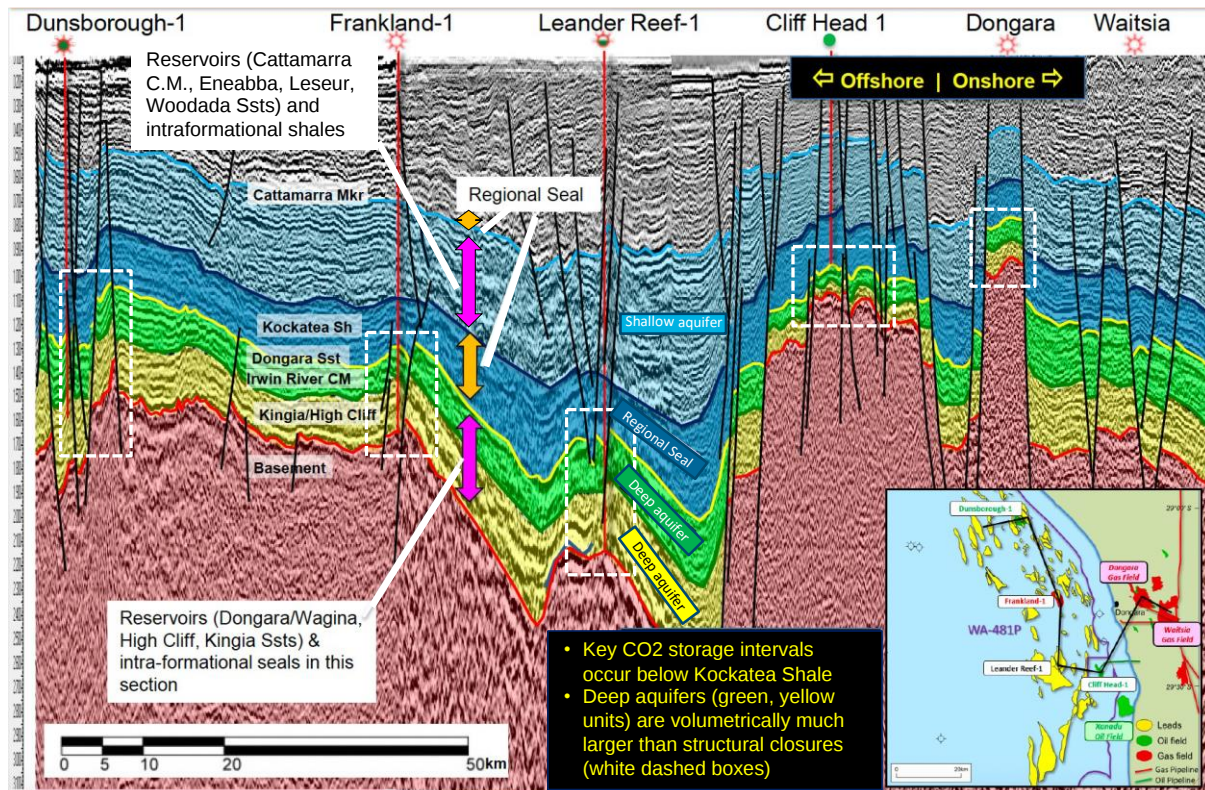
Figure 5 Composite seismic section: WA 481P CCS mechanisms
