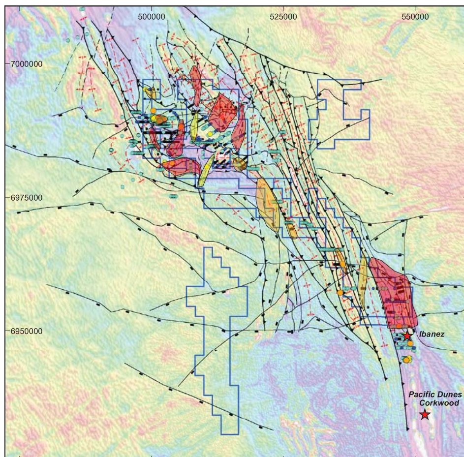
Figure 3: Structural interpretation and priority target areas along the 65km strike of greenstone belts in APC's Yamarna tenure
