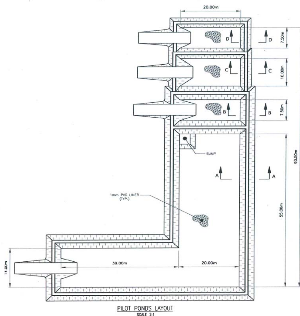
Figure 1: The pilot evaporation ponds will mirror the full-scale evaporation process with the large pre-concentration pond (A) feeding brine into the smaller crystallisation (B & C) and harvest ponds (D)
