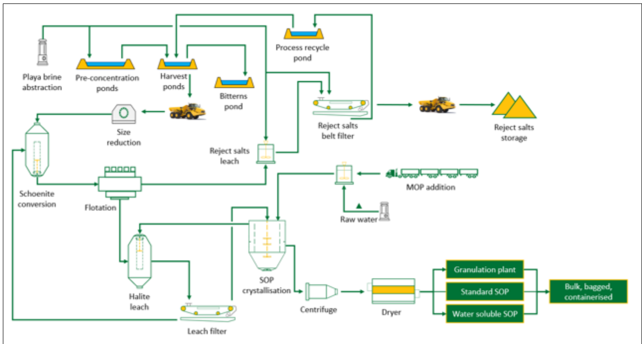
Figure 6 Process Flow Sheet
