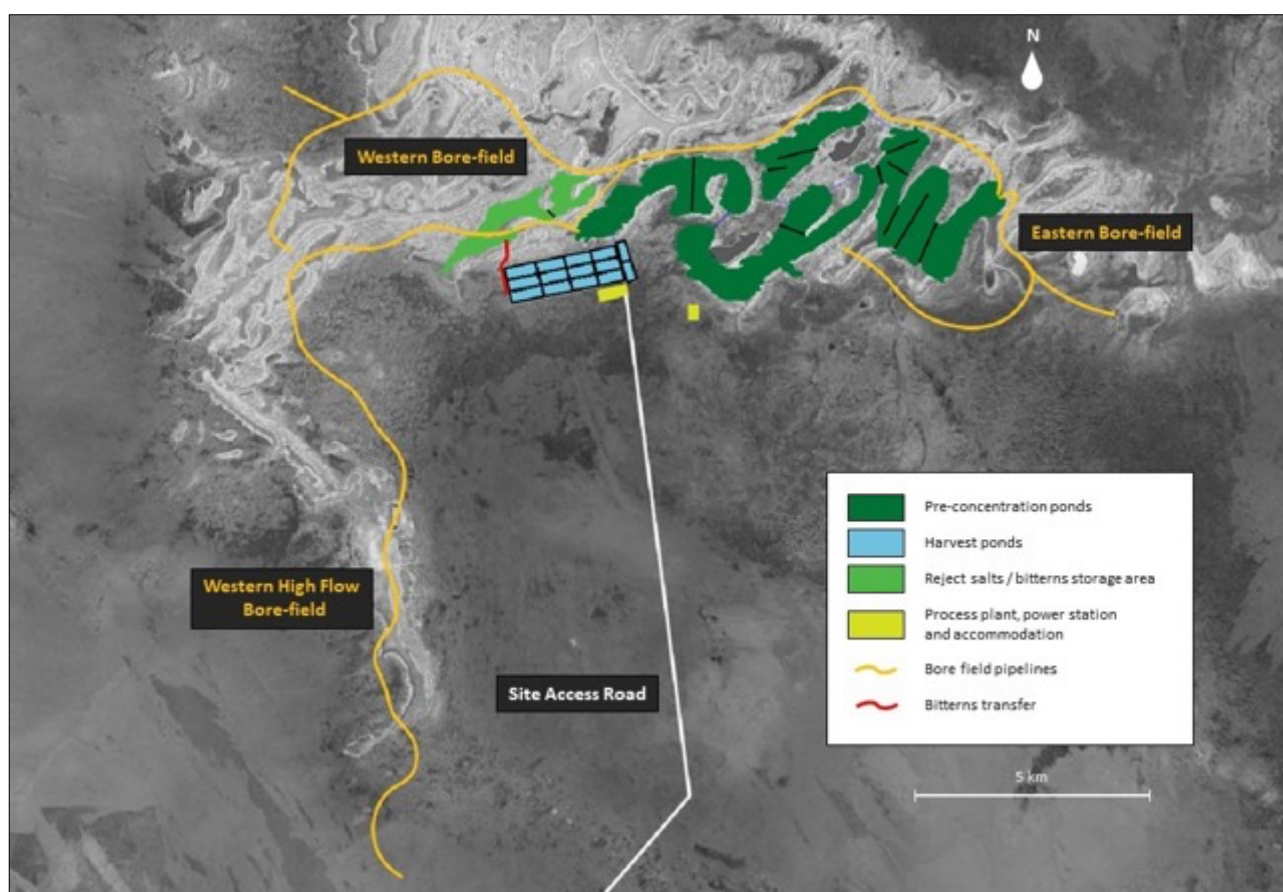
Figure 2 Site General Arrangement
