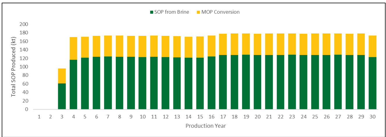
Figure 5 SOP Production Ratios
