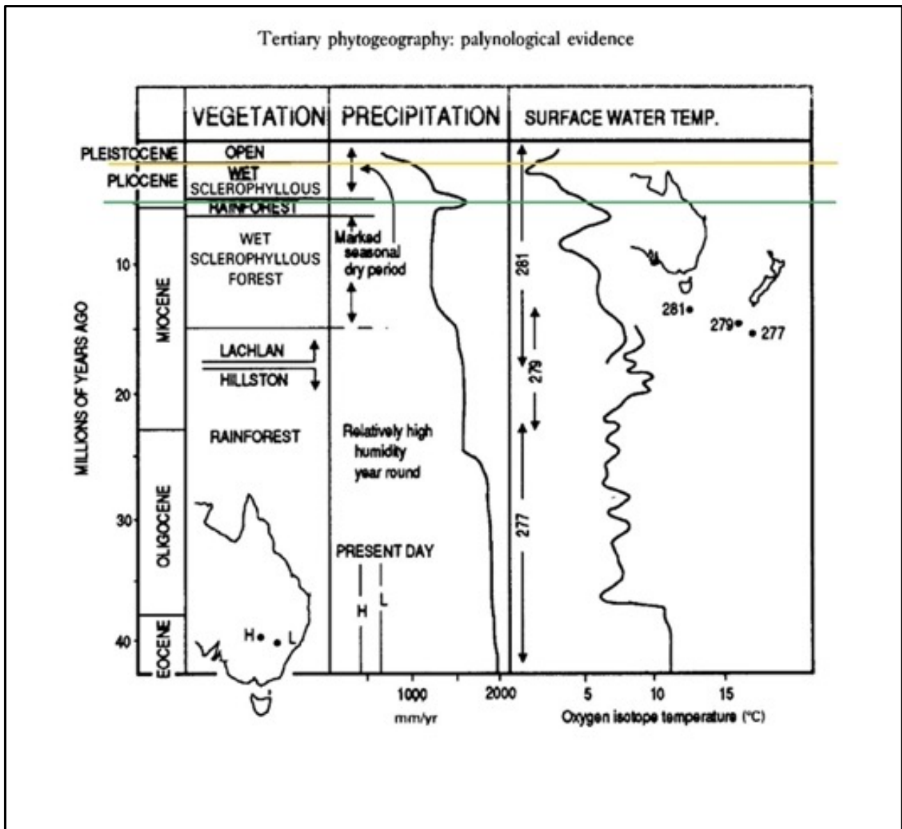
Figure 20 Outline of Tertiary Phytogeography from Martin 1994.
