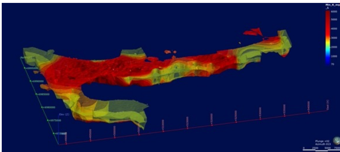
Figure 28 3D View of the Brine Resource
