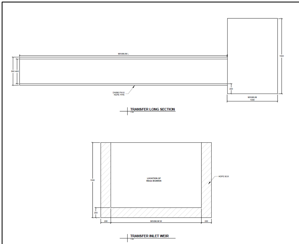
Figure 30 Typical Pipe and Culvert Configuration
