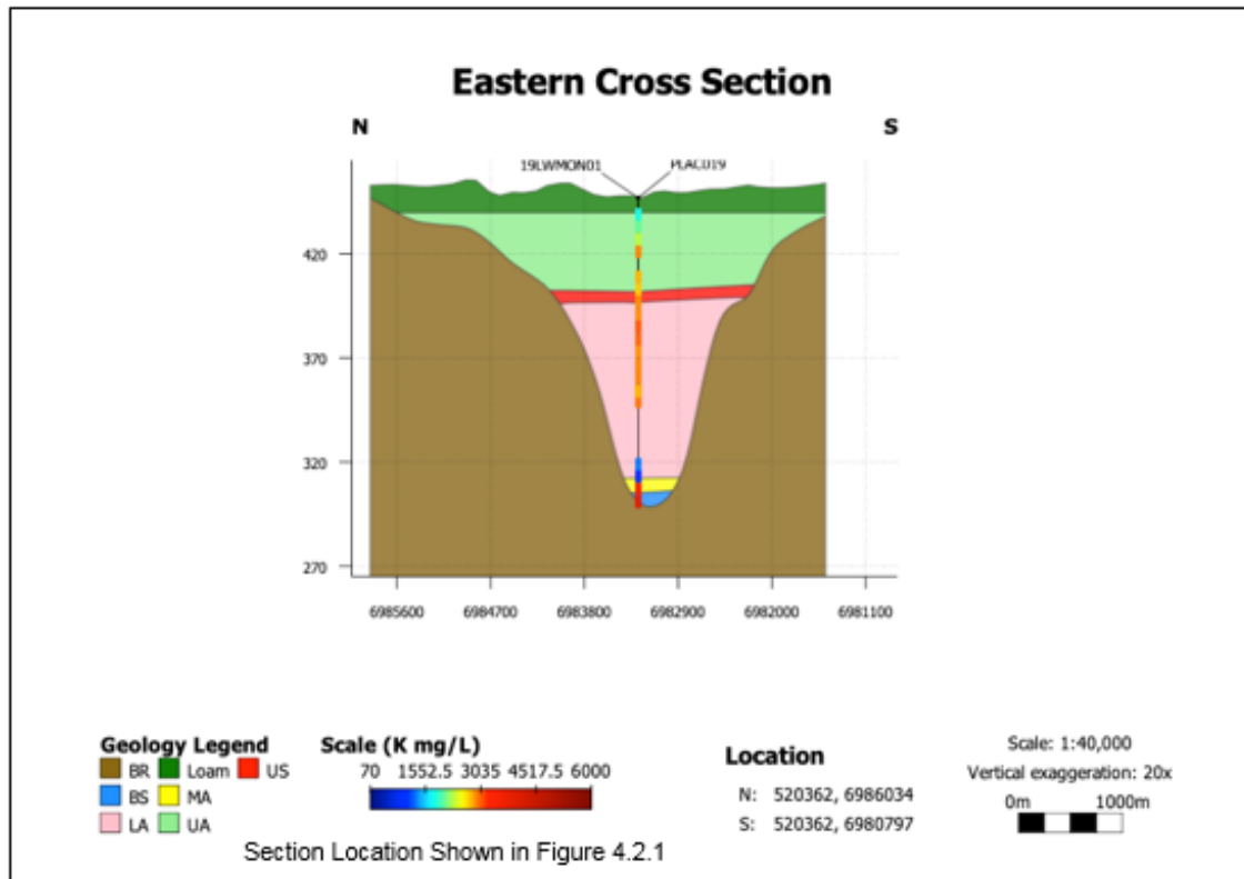
Figure 27 Eastern Cross Section
