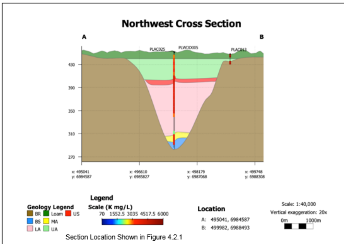
Figure 26 Northwest Cross Section
