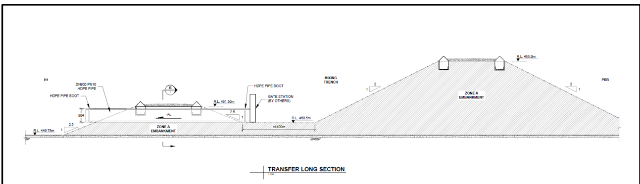
Figure 32 Typical Pipe Through Weir Configuration
