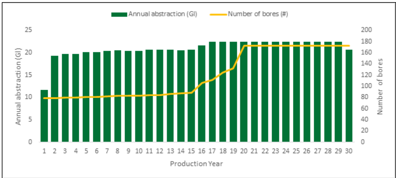
Figure 3 Brine production and bore-field expansion
