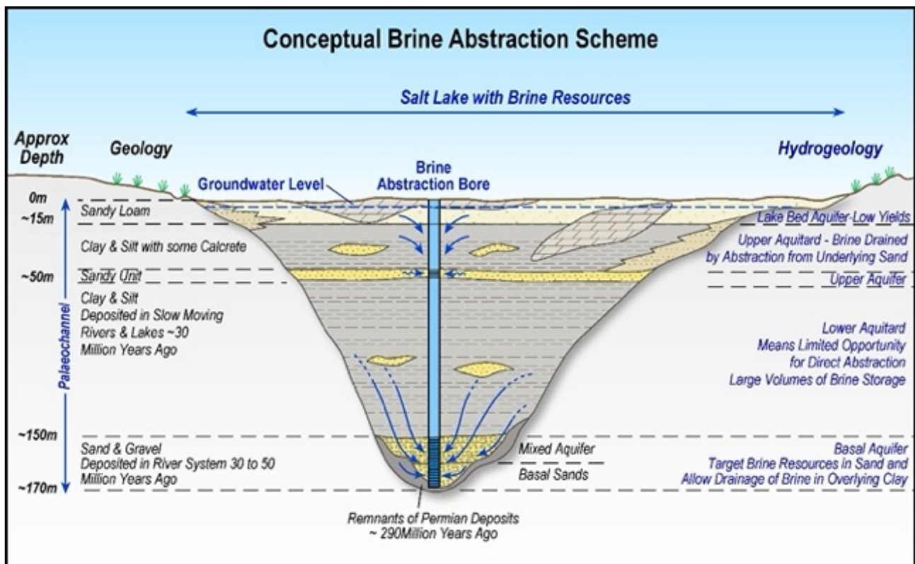
Figure 1 Conceptual palaeovalley brine abstraction scheme
