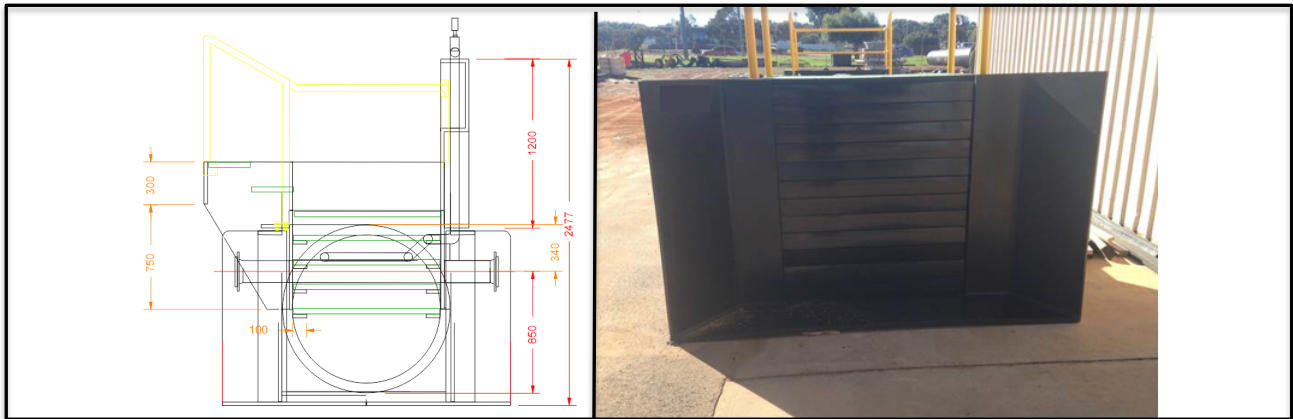
Figure 31 Typical Culvert/Weir Arrangement
