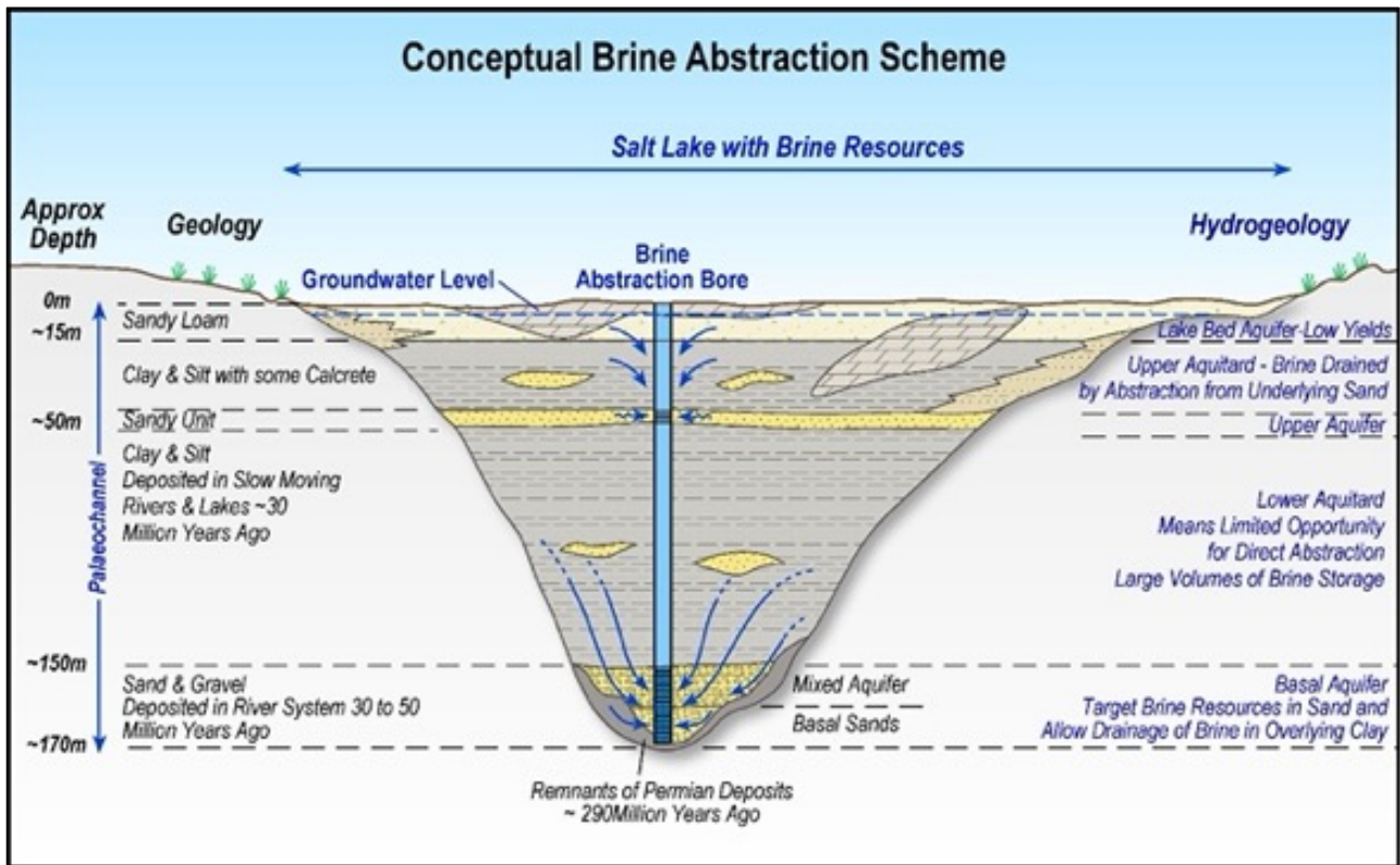
Figure 23 Conceptual Brine Abstraction Scheme
