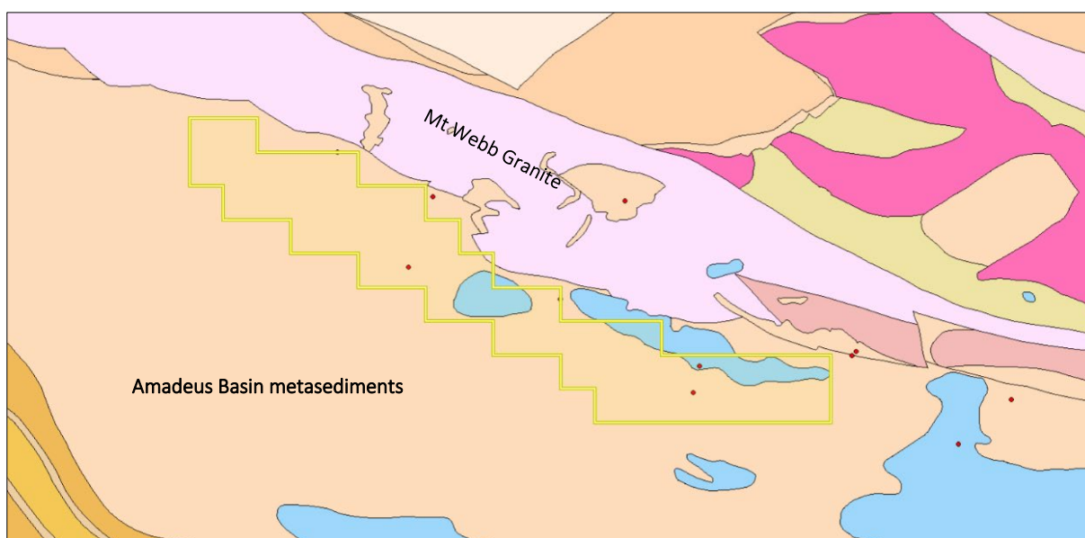
Figure 6: APC's Nexus Project bedrock geology (geophysical interpretation) & tenement E80/5778 with FQM drill collar locations
