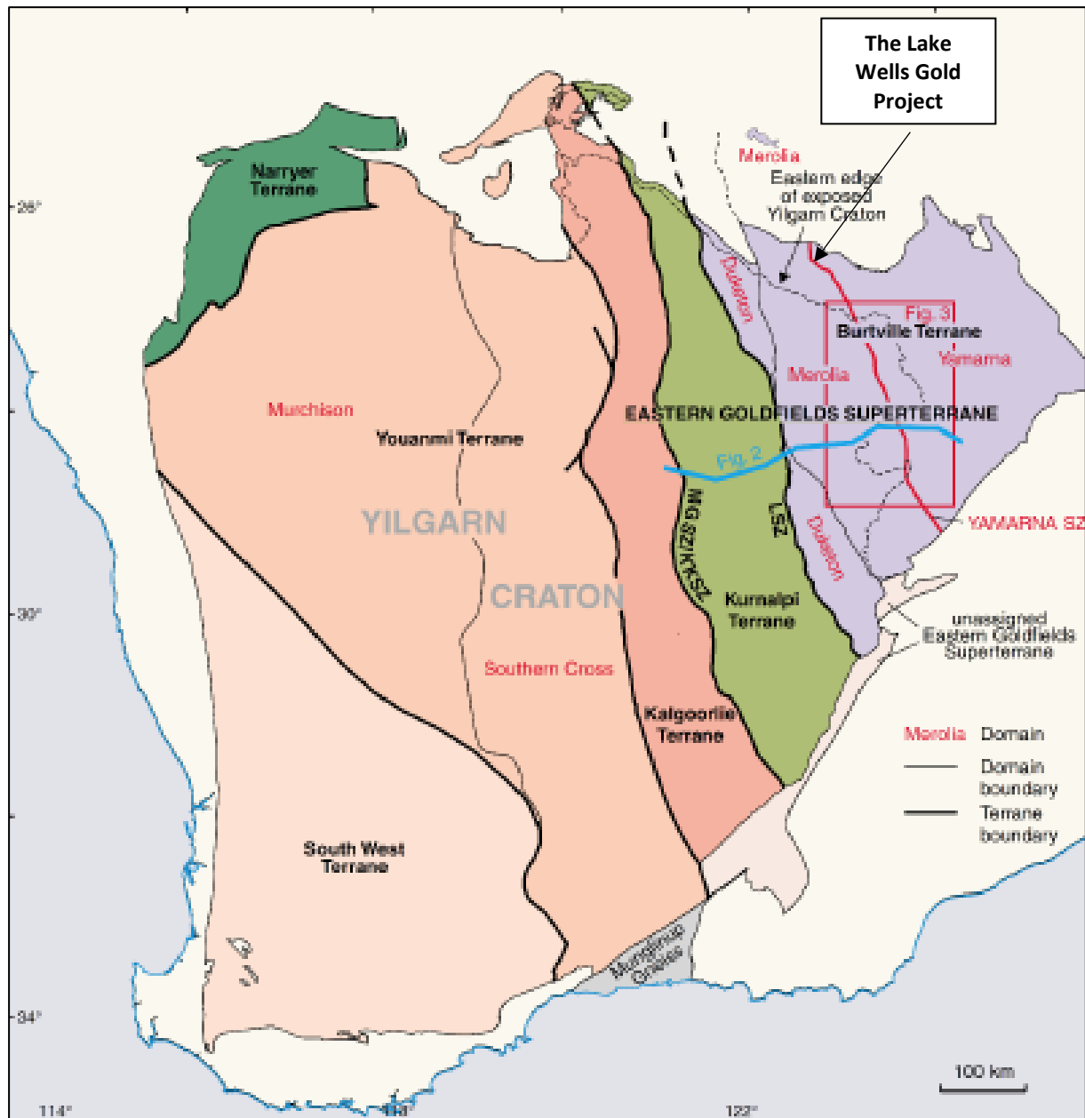
Figure 1: The Lakw Wells Gold Project sits across the Yamarna Greenstone Shear Zone on the eastern edge of the Yilgarn Craton
