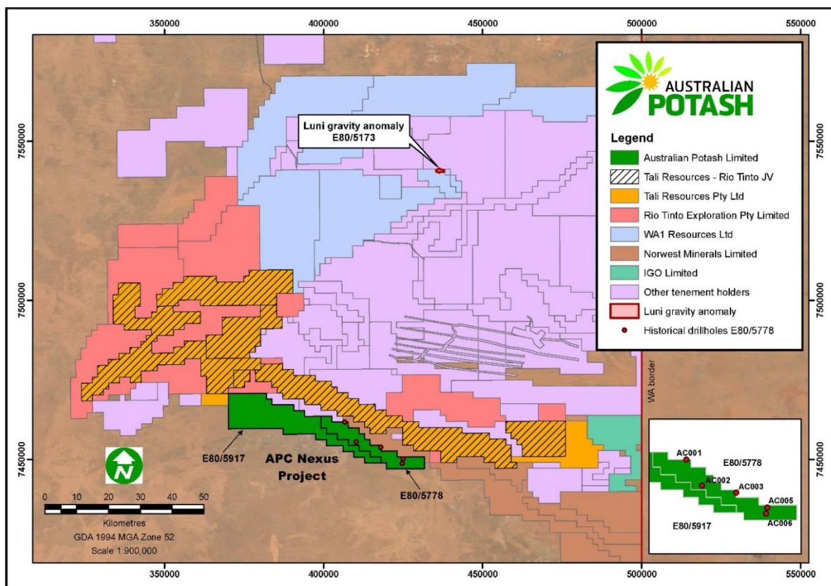
Figure 3: APC's Nexus Project location in the West Arunta region of Western Australia showing relative tenure positions of niobium discoverer WA1, Rio Tinto Exploration and IGO, and drill-hole locations of previous work conducted by FQM
