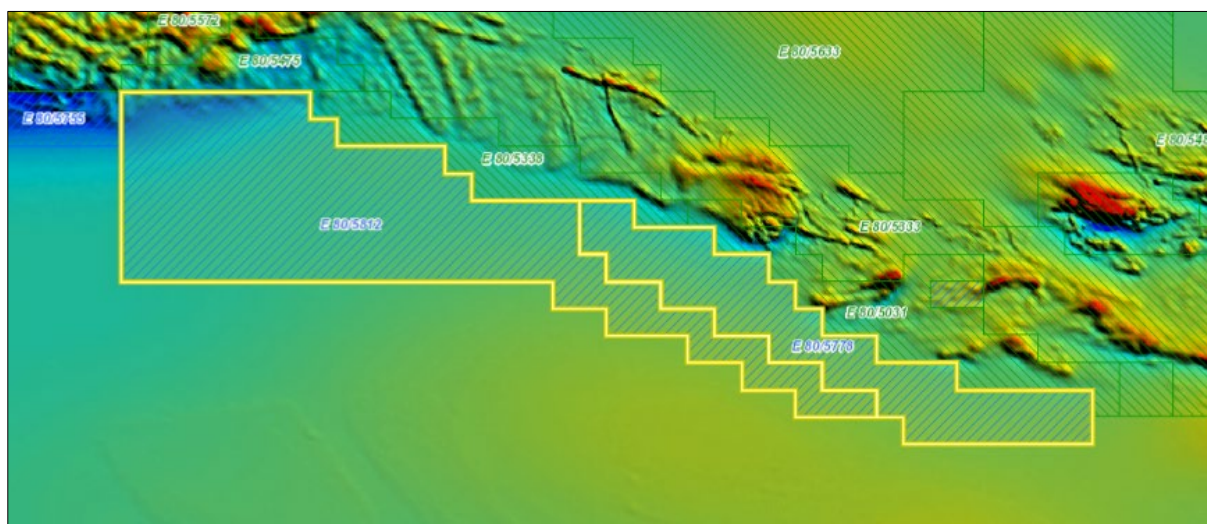
Figure 4: APC’s Nexus Project tenements overlain on magnetic image depicting the contact zone between the Webb Granite and the palaeochannel/lacustrine sediments sitting over the Amadeus Basin metasediments
