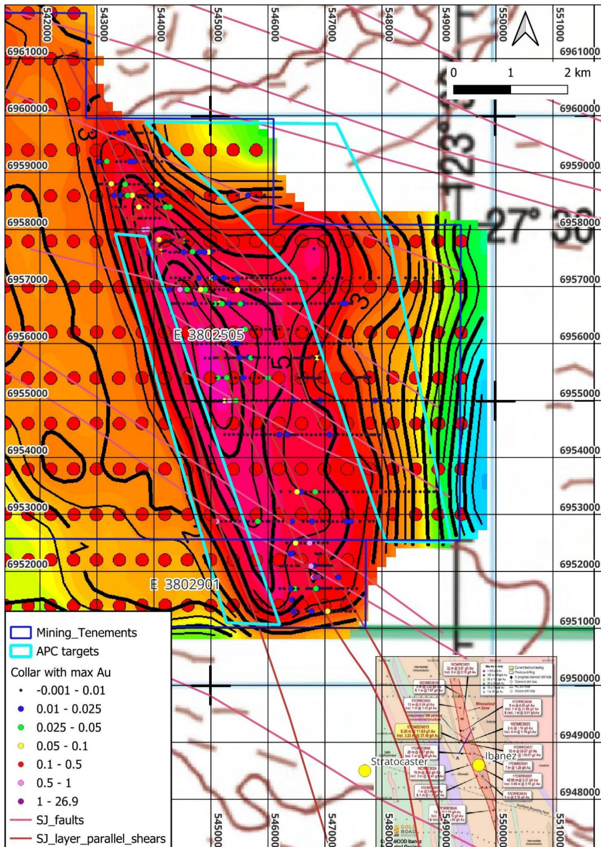
Figure 2. Gravity results showing greenstones extending west of regional drill lines.
