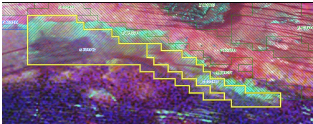
Figure 5: APC's Nexus Project tenements overlain on radiometric image depicting the contact zone between the Webb Granite and the palaeochannel/lacustrine sediments sitting over the Amadeus Basin metasediments
