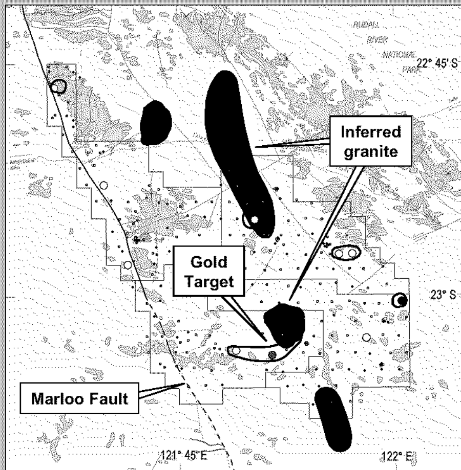
Geology
