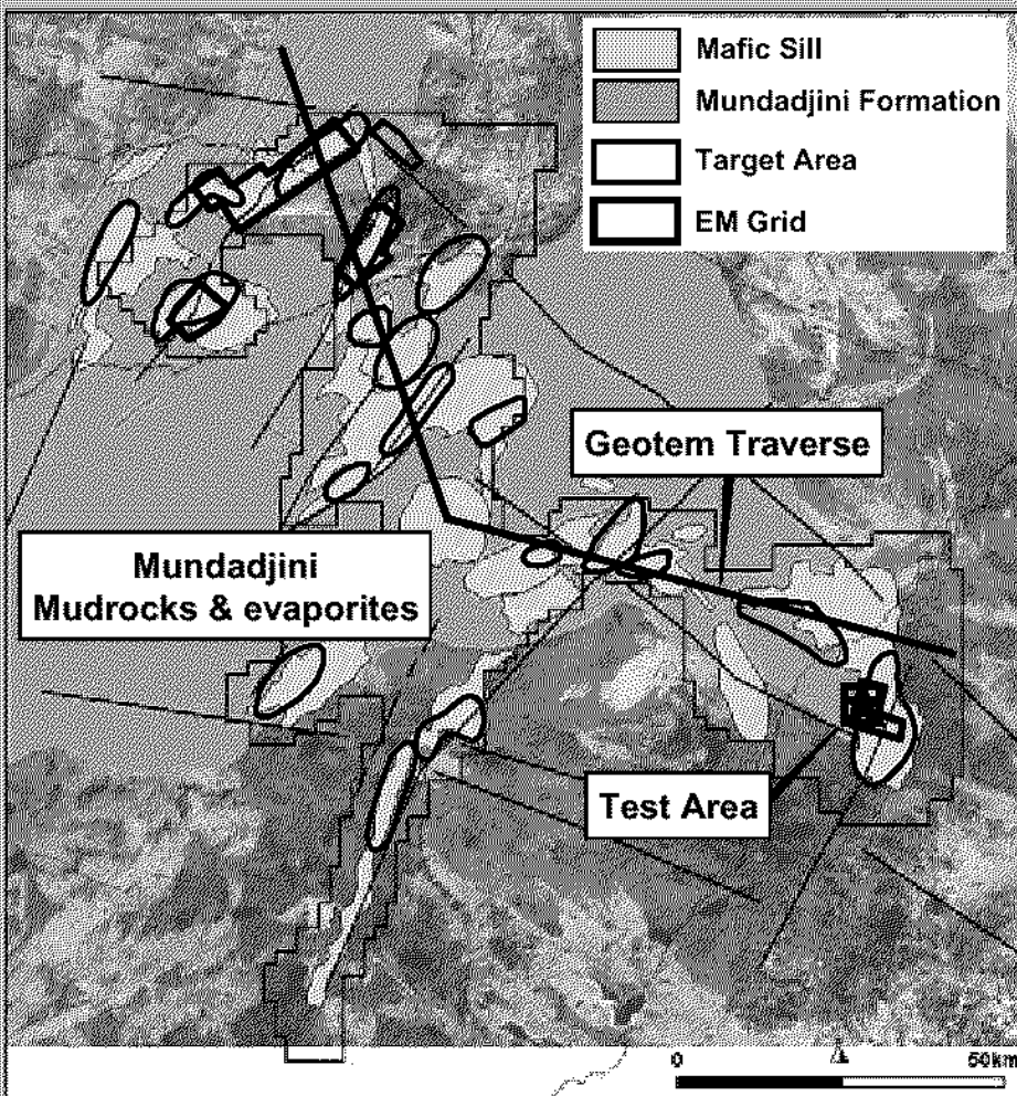
Geology
