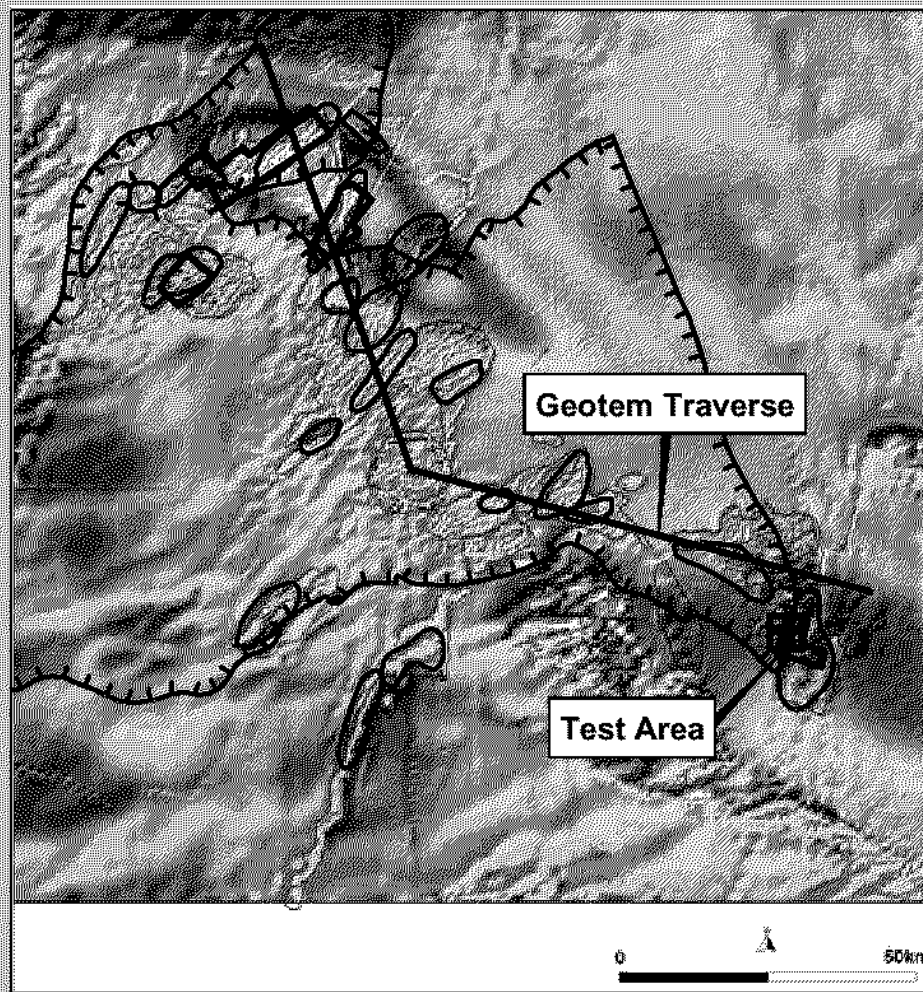
Magnetics
