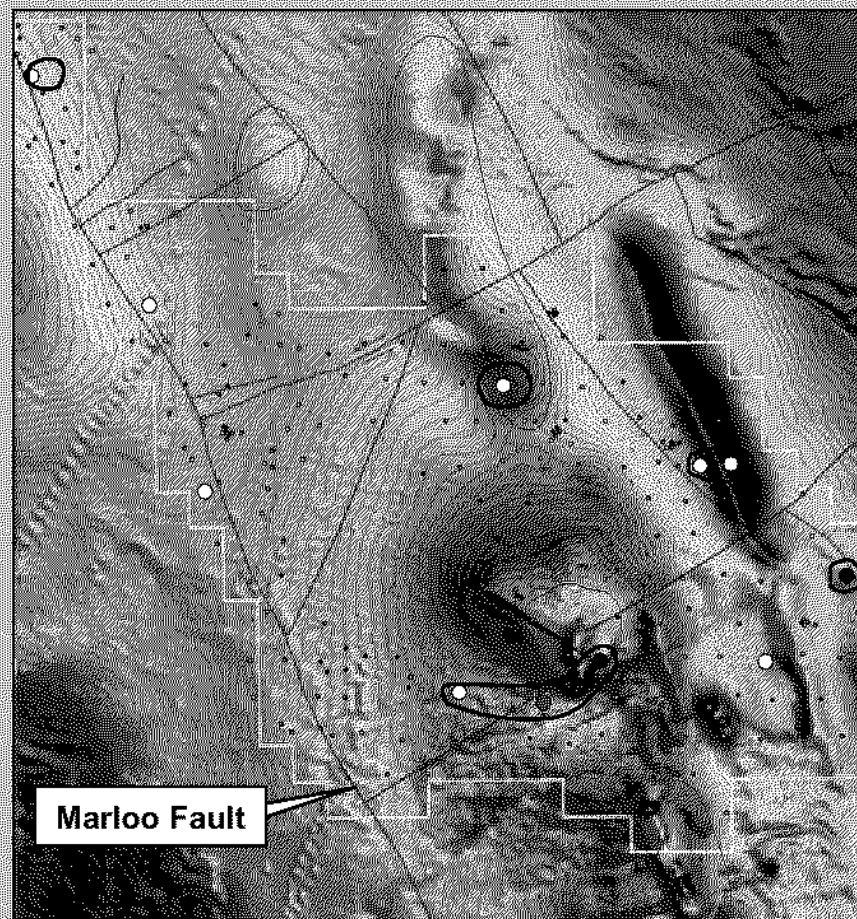
Magnetics
