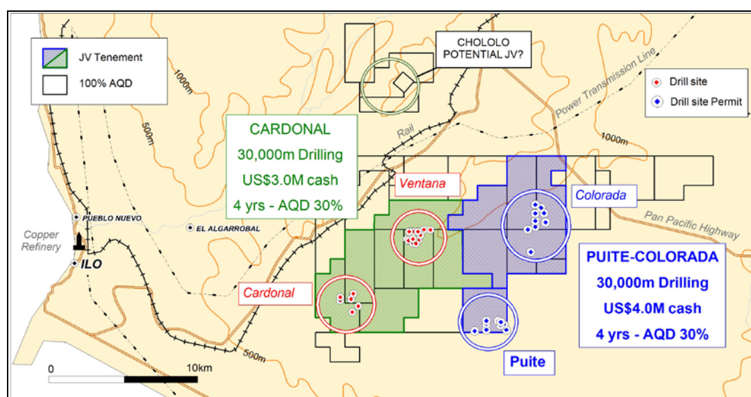
Figure 1: Prospect locations in the Ilo area
