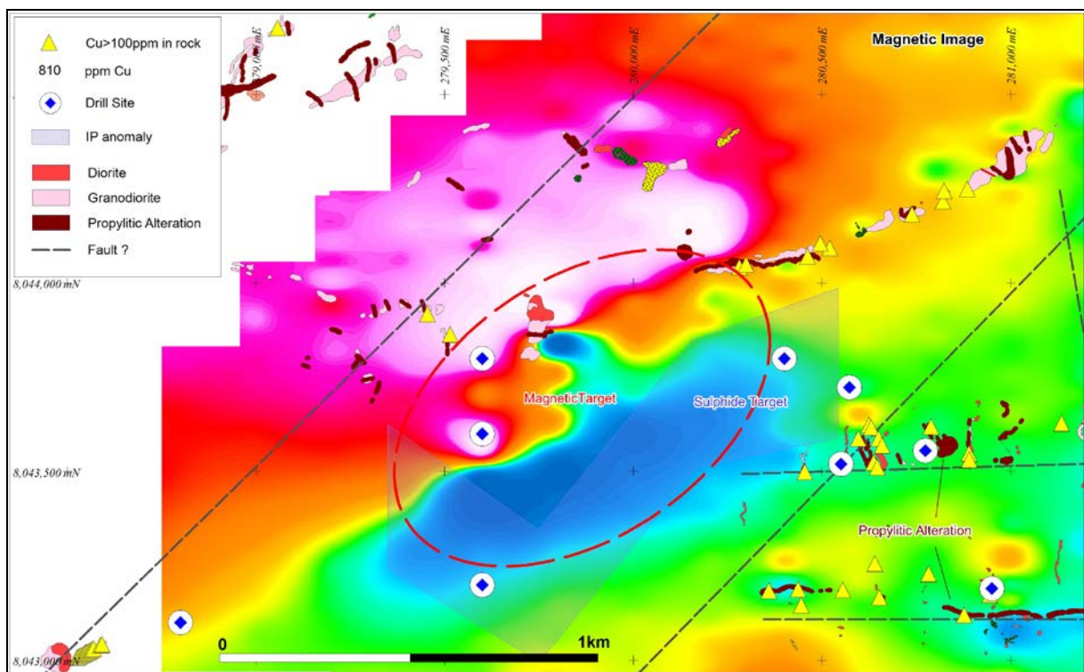
Figure 2: Puite porphyry copper-gold prospect showing magnetic and IP targets
