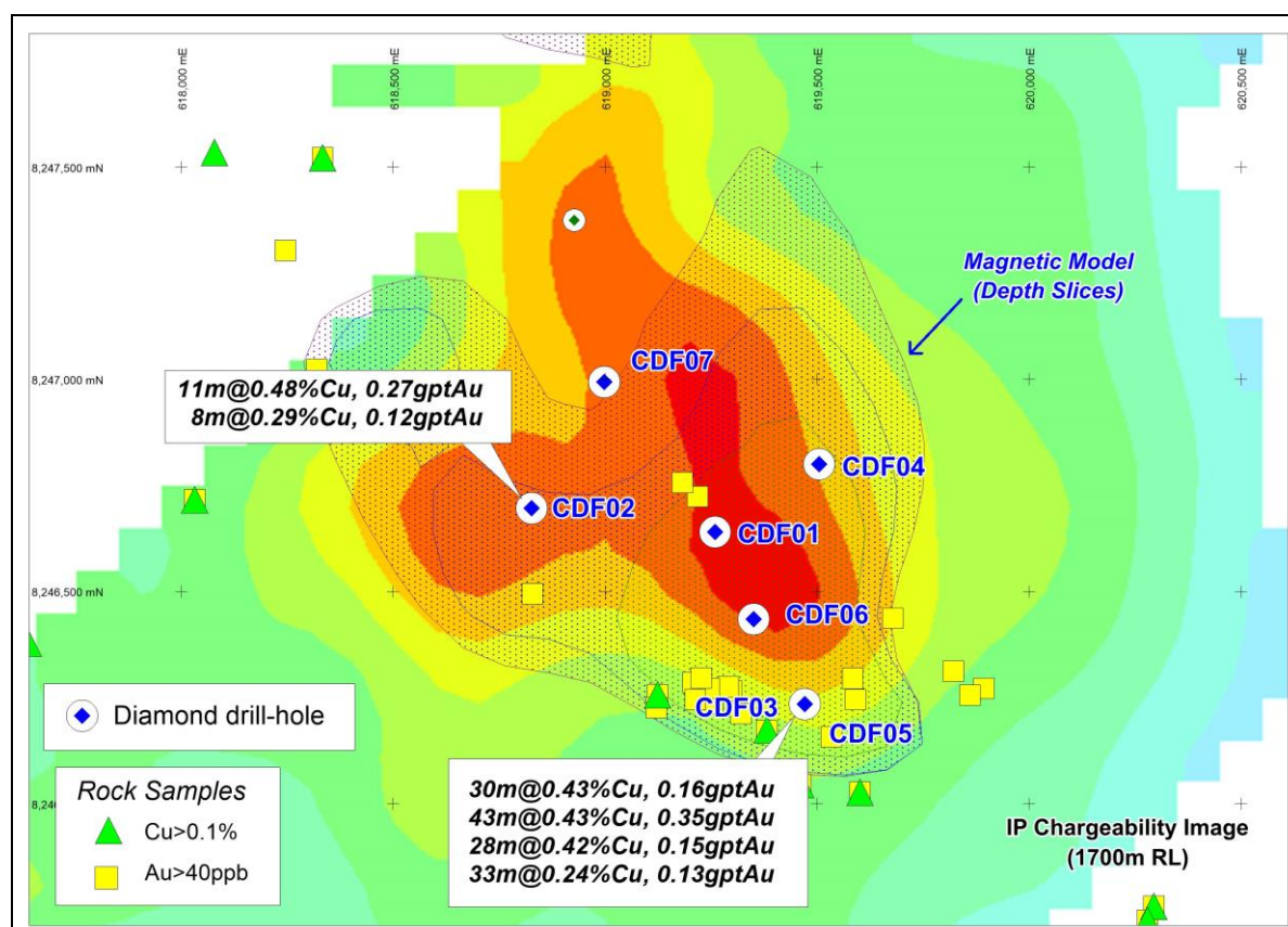
Figure 1: Cerro de Fierro IOCG target showing drill-hole locations and available assays.
