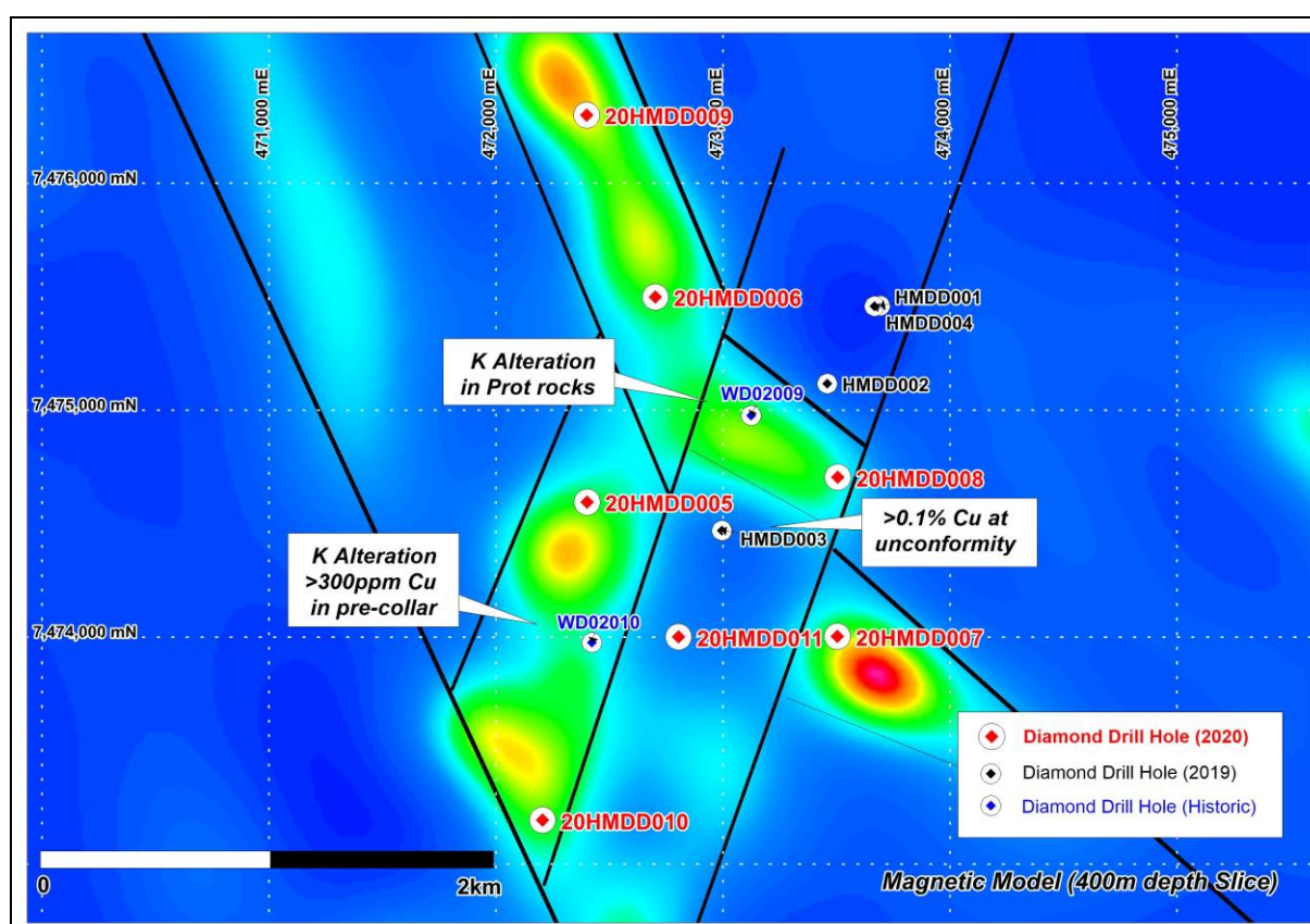
Figure 1: Hamilton Copper Prospect magnetic modelling showing the location of drill-holes.
